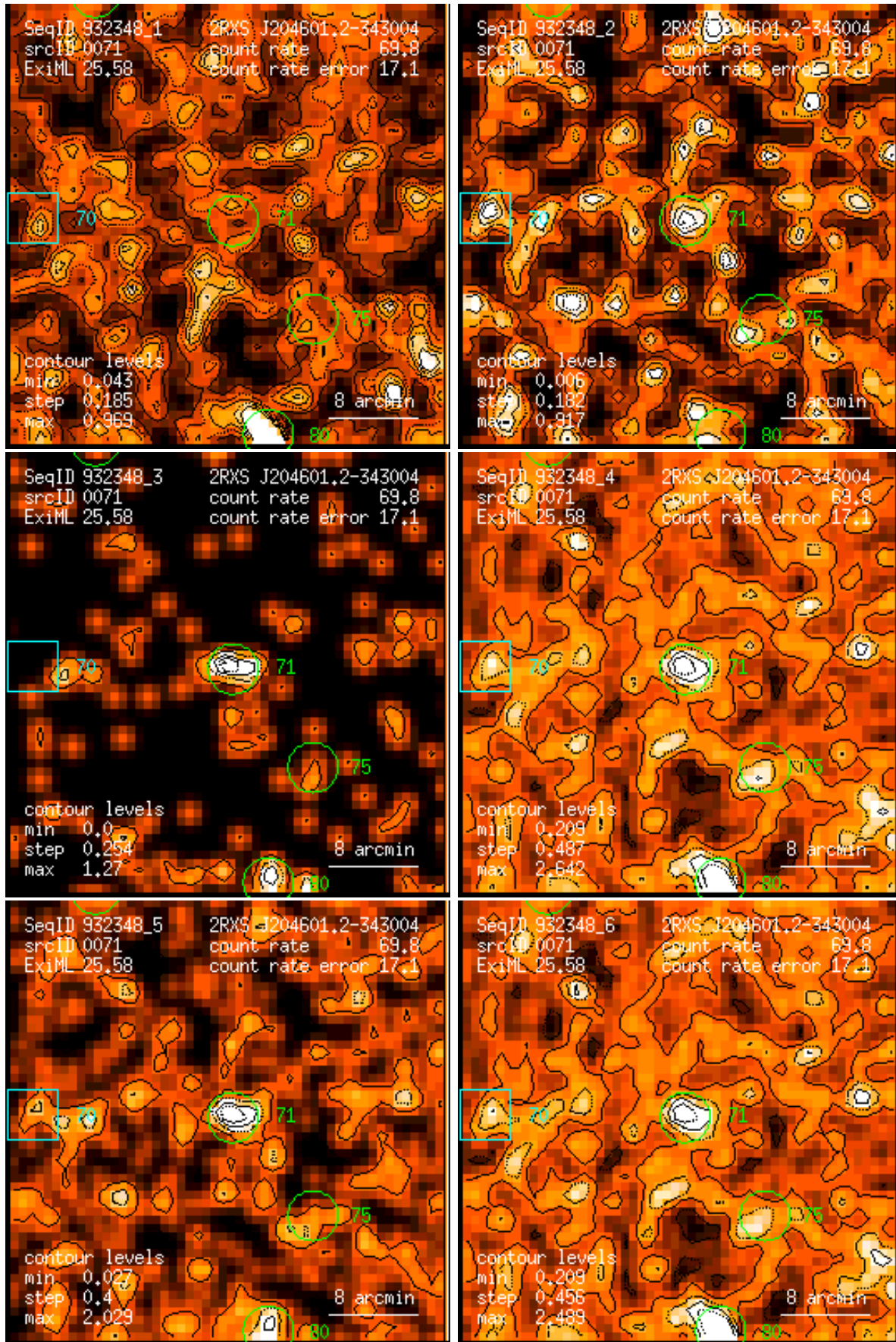
Figure 71: RASS 932348: detection 0071: band rate images, Gaussian filter: (1) PSPC channels 11 – 41, (2) 52 – 90, (3) 91 – 201, (4) 11 – 235, (5) 52 – 201, (6) 11 – 201. Broad band rates in counts/ks. Band rate contour levels in counts/ks/arcmin 2 .
