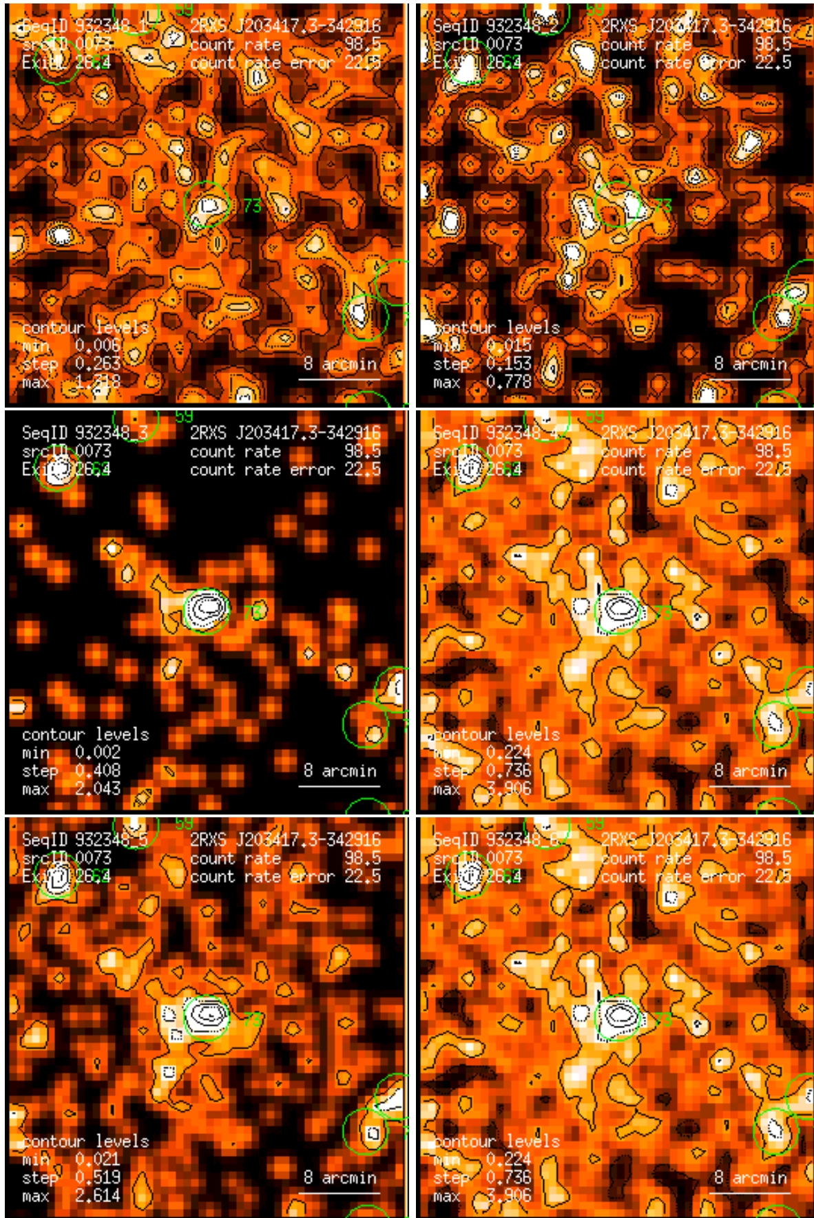
Figure 73: RASS 932348: detection 0073: band rate images, Gaussian filter: (1) PSPC channels 11 – 41, (2) 52 – 90, (3) 91 – 201, (4) 11 – 235, (5) 52 – 201, (6) 11 – 201. Broad band rates in counts/ks. Band rate contour levels in counts/ks/arcmin 2 .
