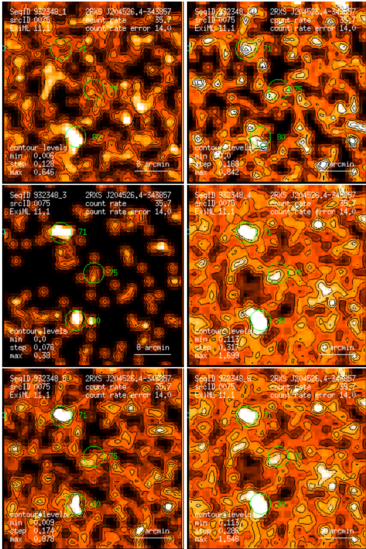
Figure 75: RASS 932348: detection 0075: band rate images, Gaussian filter: (1) PSPC channels 11 – 41, (2) 52 – 90, (3) 91 – 201, (4) 11 – 235, (5) 52 – 201, (6) 11 – 201. Broad band rates in counts/ks. Band rate contour levels in counts/ks/arcmin 2 .
