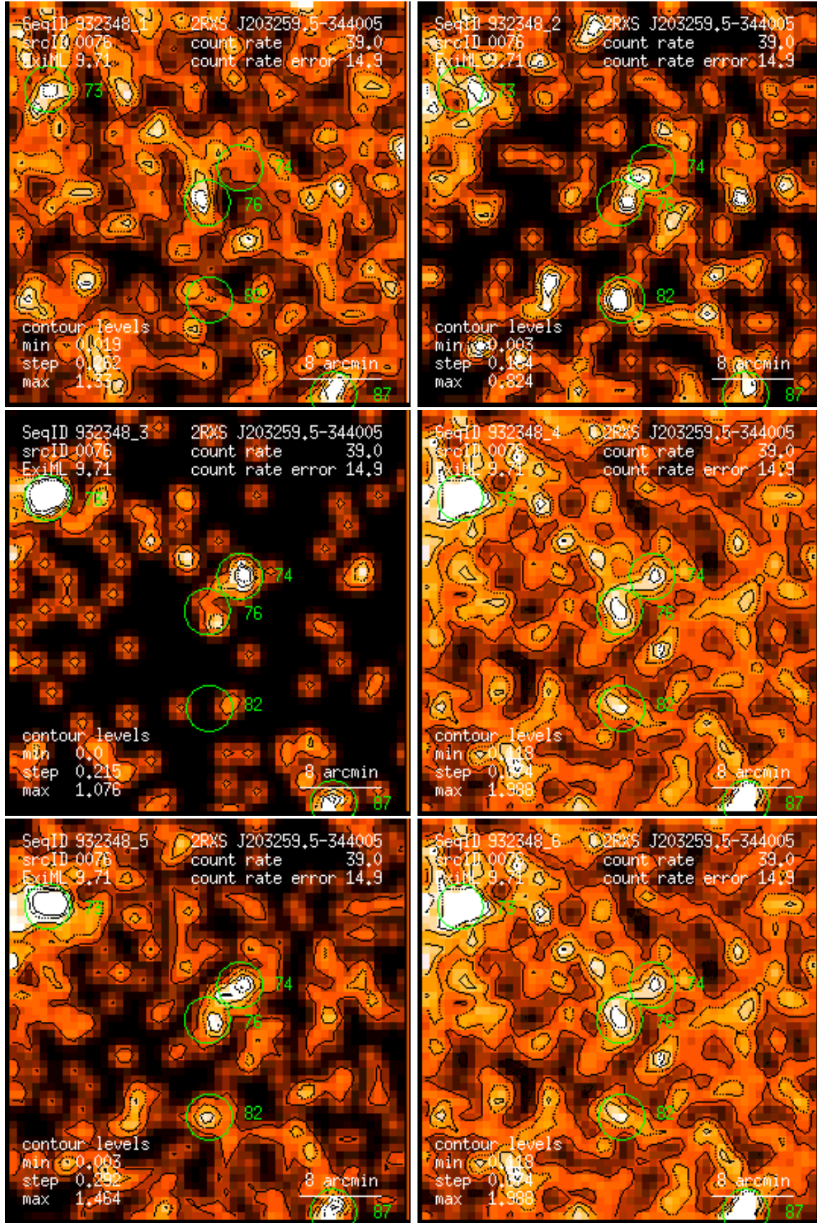
Figure 76: RASS 932348: detection 0076: band rate images, Gaussian filter: (1) PSPC channels 11 – 41, (2) 52 – 90, (3) 91 – 201, (4) 11 – 235, (5) 52 – 201, (6) 11 – 201. Broad band rates in counts/ks. Band rate contour levels in counts/ks/arcmin 2 .
