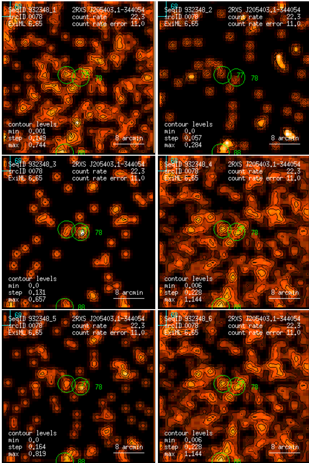
Figure 78: RASS 932348: detection 0078: band rate images, Gaussian filter: (1) PSPC channels 11 – 41, (2) 52 – 90, (3) 91 – 201, (4) 11 – 235, (5) 52 – 201, (6) 11 – 201. Broad band rates in counts/ks. Band rate contour levels in counts/ks/arcmin 2 .
