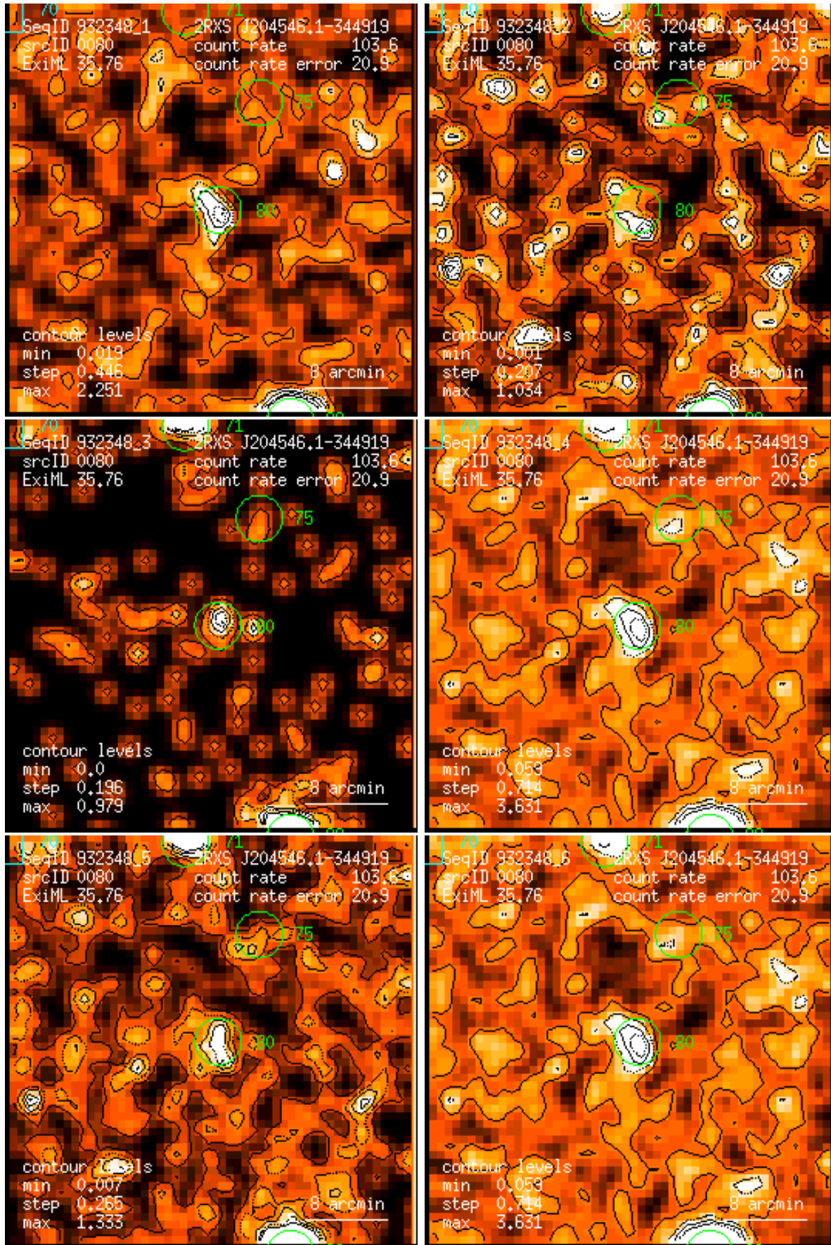
Figure 80: RASS 932348: detection 0080: band rate images, Gaussian filter: (1) PSPC channels 11 – 41, (2) 52 – 90, (3) 91 – 201, (4) 11 – 235, (5) 52 – 201, (6) 11 – 201. Broad band rates in counts/ks. Band rate contour levels in counts/ks/arcmin 2 .
