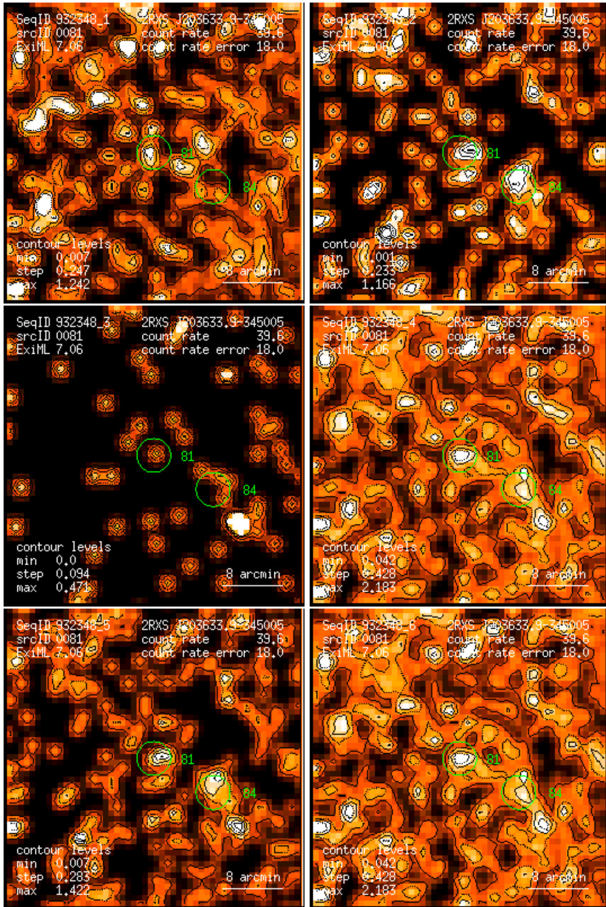
Figure 81: RASS 932348: detection 0081: band rate images, Gaussian filter: (1) PSPC channels 11 – 41, (2) 52 – 90, (3) 91 – 201, (4) 11 – 235, (5) 52 – 201, (6) 11 – 201. Broad band rates in counts/ks. Band rate contour levels in counts/ks/arcmin 2 .
