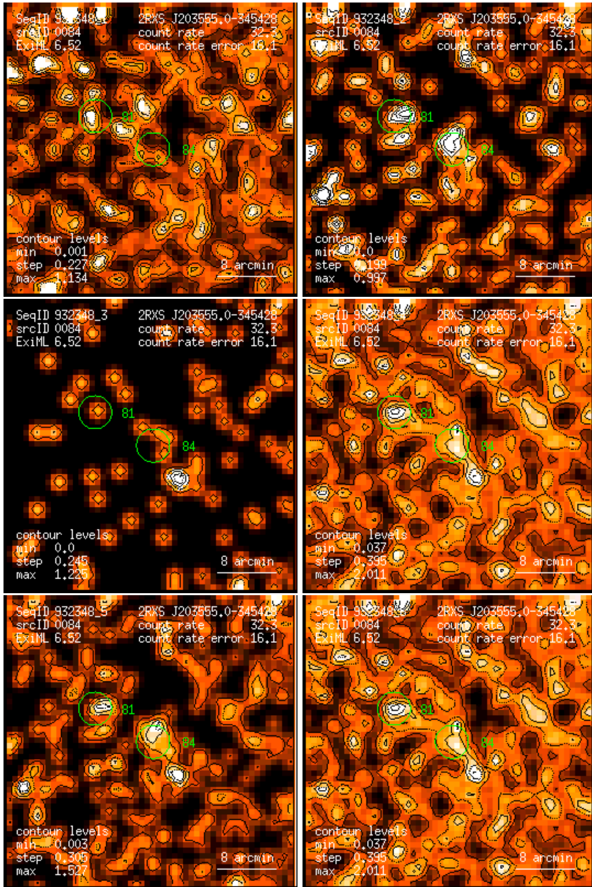
Figure 84: RASS 932348: detection 0084: band rate images, Gaussian filter: (1) PSPC channels 11 – 41, (2) 52 – 90, (3) 91 – 201, (4) 11 – 235, (5) 52 – 201, (6) 11 – 201. Broad band rates in counts/ks. Band rate contour levels in counts/ks/arcmin 2 .
