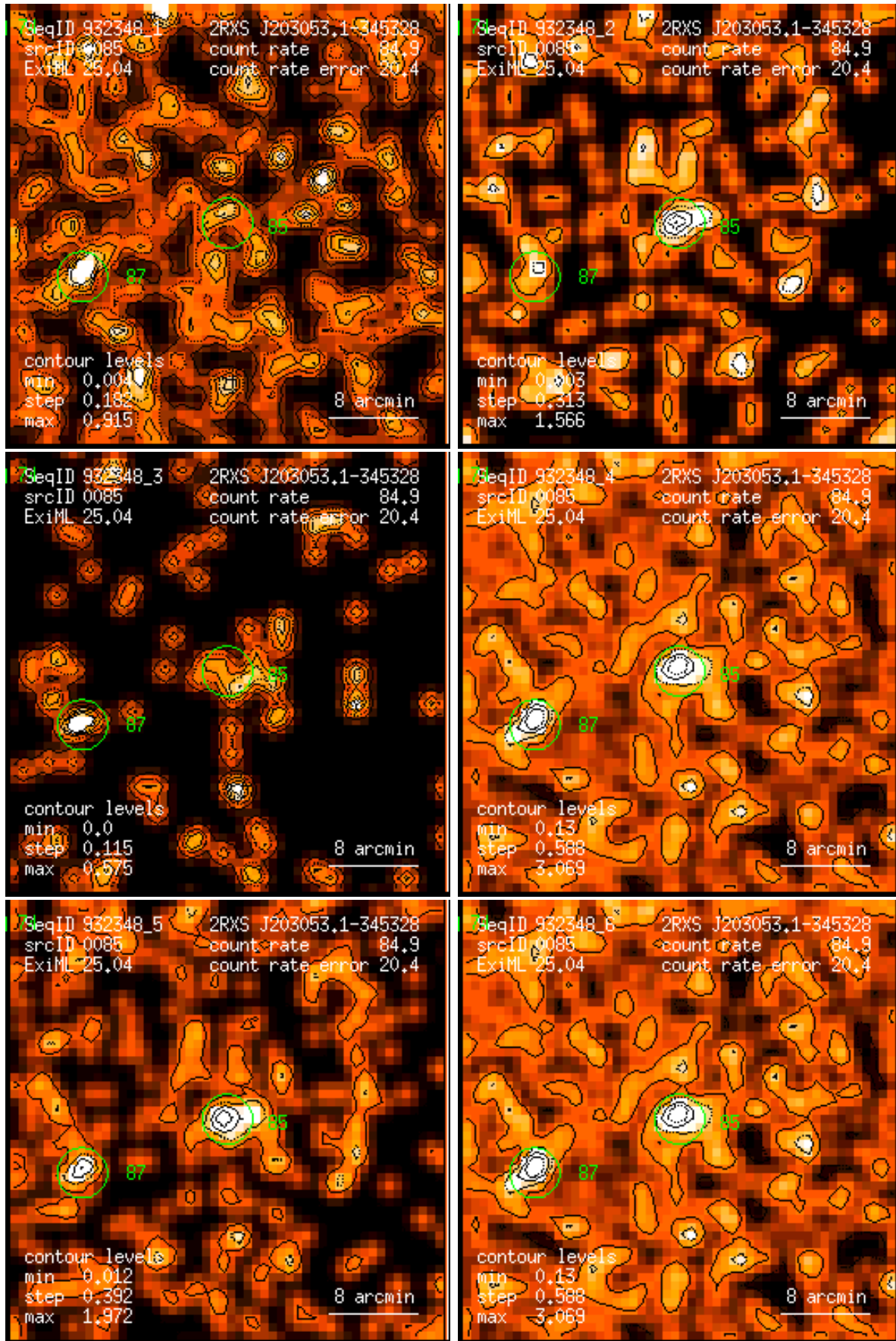
Figure 85: RASS 932348: detection 0085: band rate images, Gaussian filter: (1) PSPC channels 11 – 41, (2) 52 – 90, (3) 91 – 201, (4) 11 – 235, (5) 52 – 201, (6) 11 – 201. Broad band rates in counts/ks. Band rate contour levels in counts/ks/arcmin 2 .
