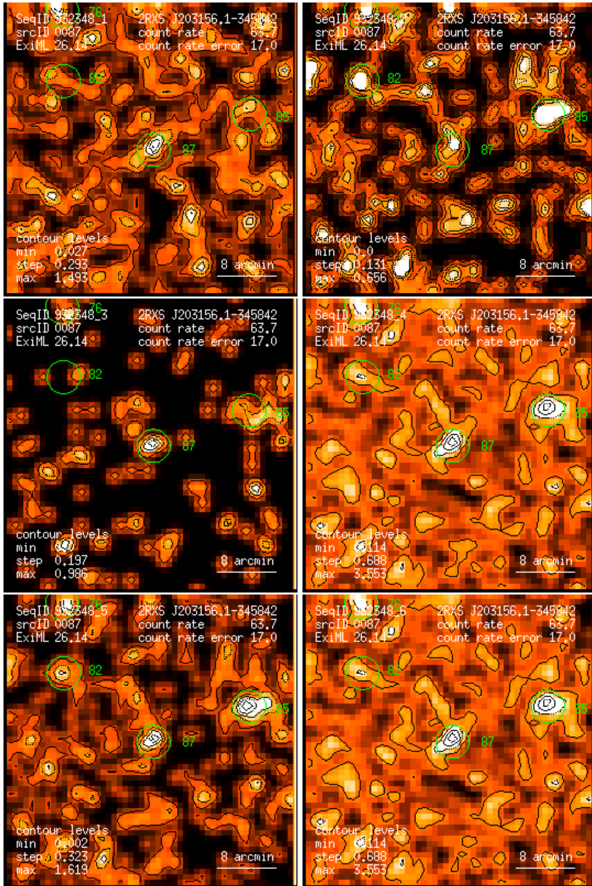
Figure 87: RASS 932348: detection 0087: band rate images, Gaussian filter: (1) PSPC channels 11 – 41, (2) 52 – 90, (3) 91 – 201, (4) 11 – 235, (5) 52 – 201, (6) 11 – 201. Broad band rates in counts/ks. Band rate contour levels in counts/ks/arcmin 2 .
