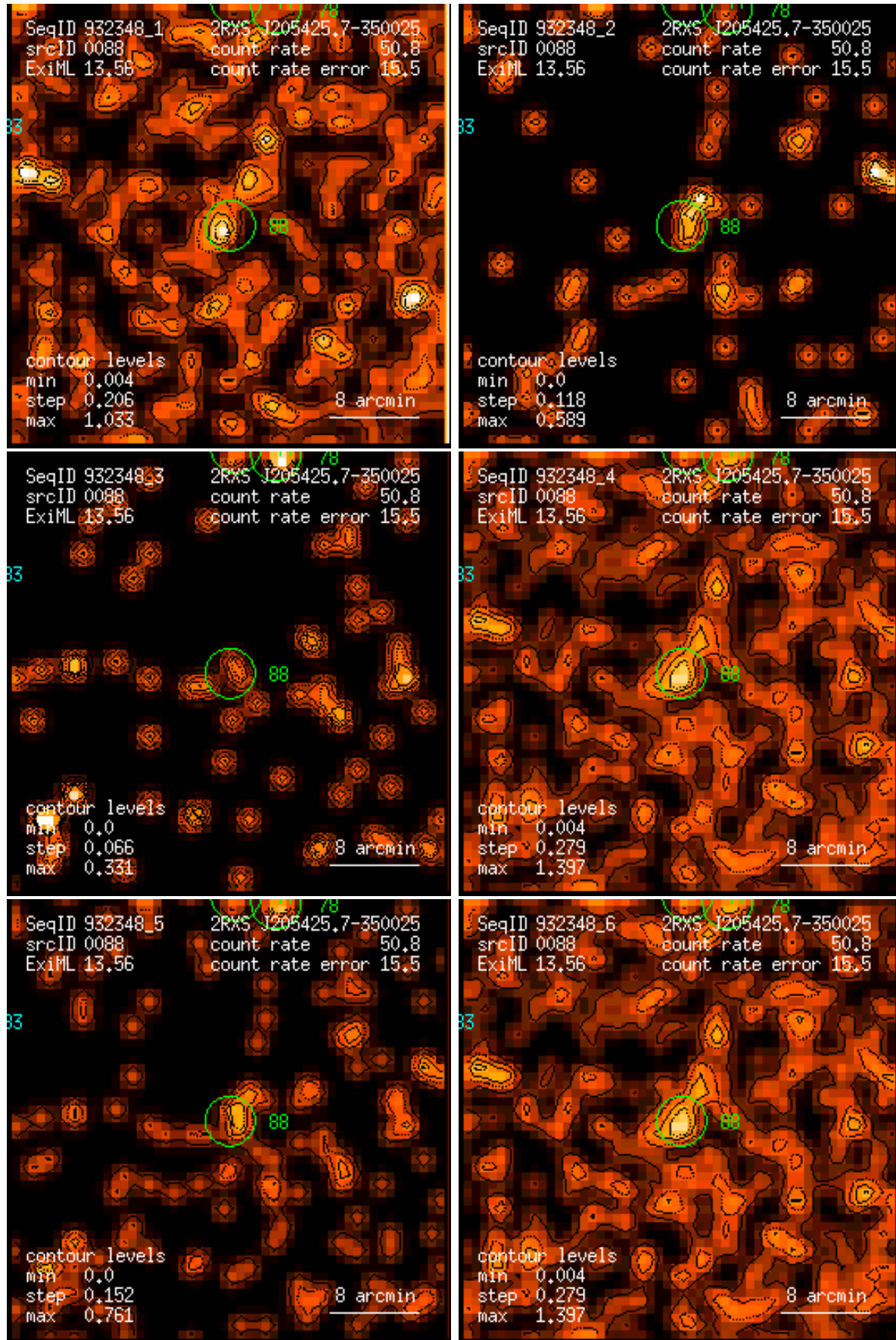
Figure 88: RASS 932348: detection 0088: band rate images, Gaussian filter: (1) PSPC channels 11 – 41, (2) 52 – 90, (3) 91 – 201, (4) 11 – 235, (5) 52 – 201, (6) 11 – 201. Broad band rates in counts/ks. Band rate contour levels in counts/ks/arcmin 2 .
