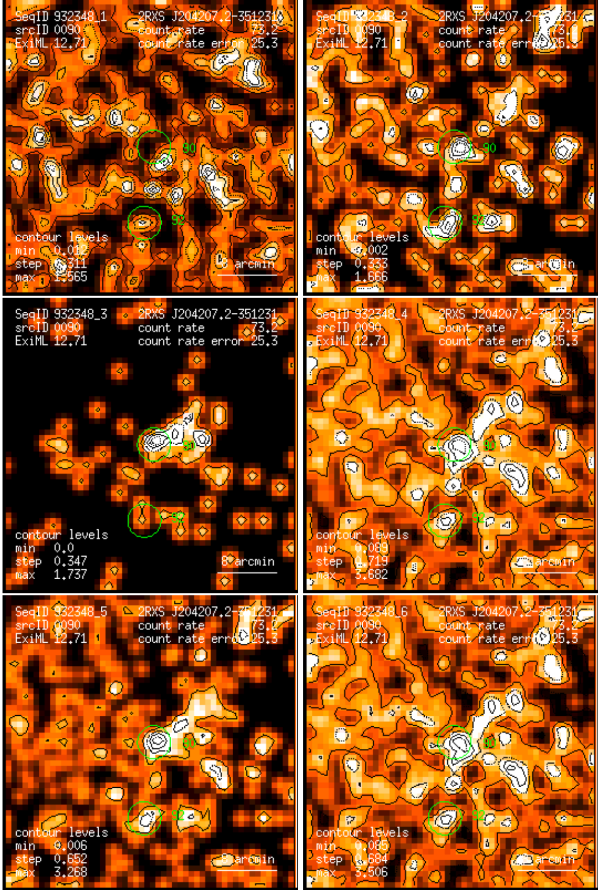
Figure 90: RASS 932348: detection 0090: band rate images, Gaussian filter: (1) PSPC channels 11 – 41, (2) 52 – 90, (3) 91 – 201, (4) 11 – 235, (5) 52 – 201, (6) 11 – 201. Broad band rates in counts/ks. Band rate contour levels in counts/ks/arcmin 2 .
