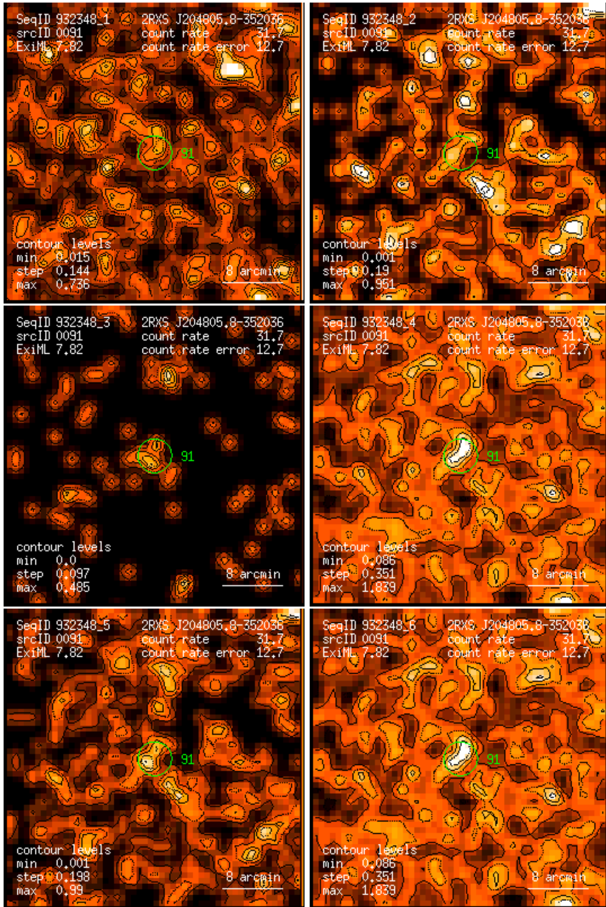
Figure 91: RASS 932348: detection 0091: band rate images, Gaussian filter: (1) PSPC channels 11 – 41, (2) 52 – 90, (3) 91 – 201, (4) 11 – 235, (5) 52 – 201, (6) 11 – 201. Broad band rates in counts/ks. Band rate contour levels in counts/ks/arcmin 2 .
