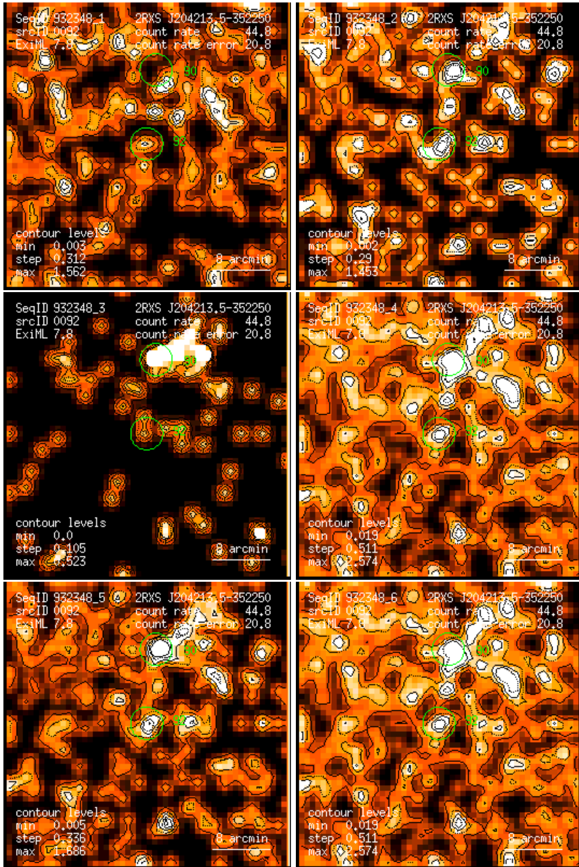
Figure 92: RASS 932348: detection 0092: band rate images, Gaussian filter: (1) PSPC channels 11 – 41, (2) 52 – 90, (3) 91 – 201, (4) 11 – 235, (5) 52 – 201, (6) 11 – 201. Broad band rates in counts/ks. Band rate contour levels in counts/ks/arcmin 2 .
