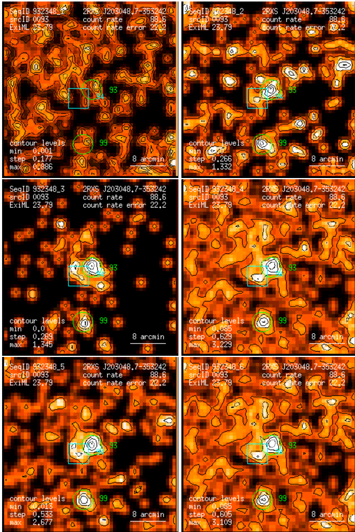
Figure 93: RASS 932348: detection 0093: band rate images, Gaussian filter: (1) PSPC channels 11 – 41, (2) 52 – 90, (3) 91 – 201, (4) 11 – 235, (5) 52 – 201, (6) 11 – 201. Broad band rates in counts/ks. Band rate contour levels in counts/ks/arcmin 2 .
