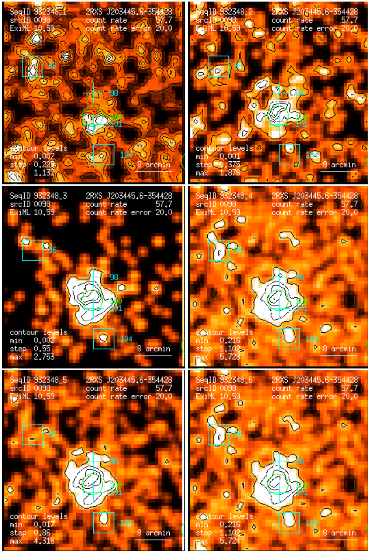
Figure 98: RASS 932348: detection 0098: band rate images, Gaussian filter: (1) PSPC channels 11 – 41, (2) 52 – 90, (3) 91 – 201, (4) 11 – 235, (5) 52 – 201, (6) 11 – 201. Broad band rates in counts/ks. Band rate contour levels in counts/ks/arcmin 2 .
