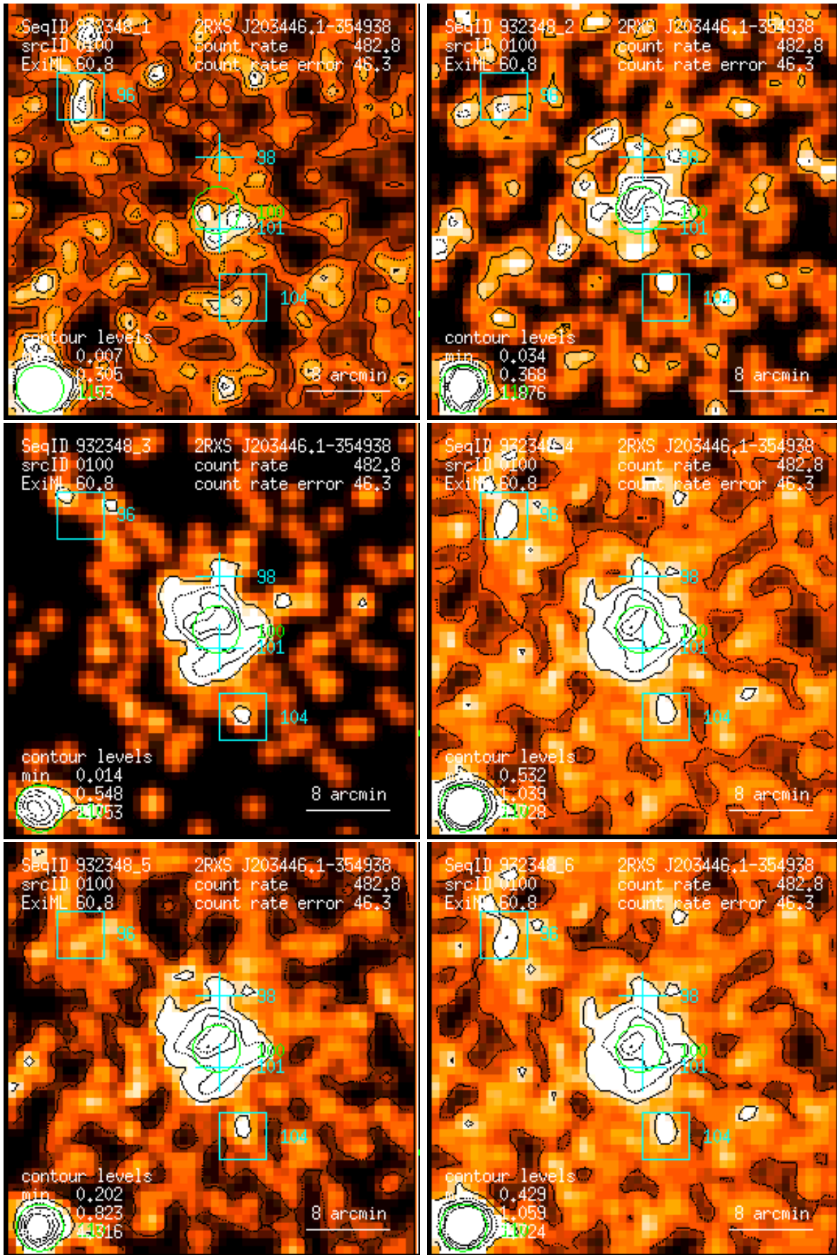
Figure 100: RASS 932348: detection 0100: band rate images, Gaussian filter: (1) PSPC channels 11 – 41, (2) 52 – 90, (3) 91 – 201, (4) 11 – 235, (5) 52 – 201, (6) 11 – 201. Broad band rates in counts/ks. Band rate contour levels in counts/ks/arcmin 2 .
