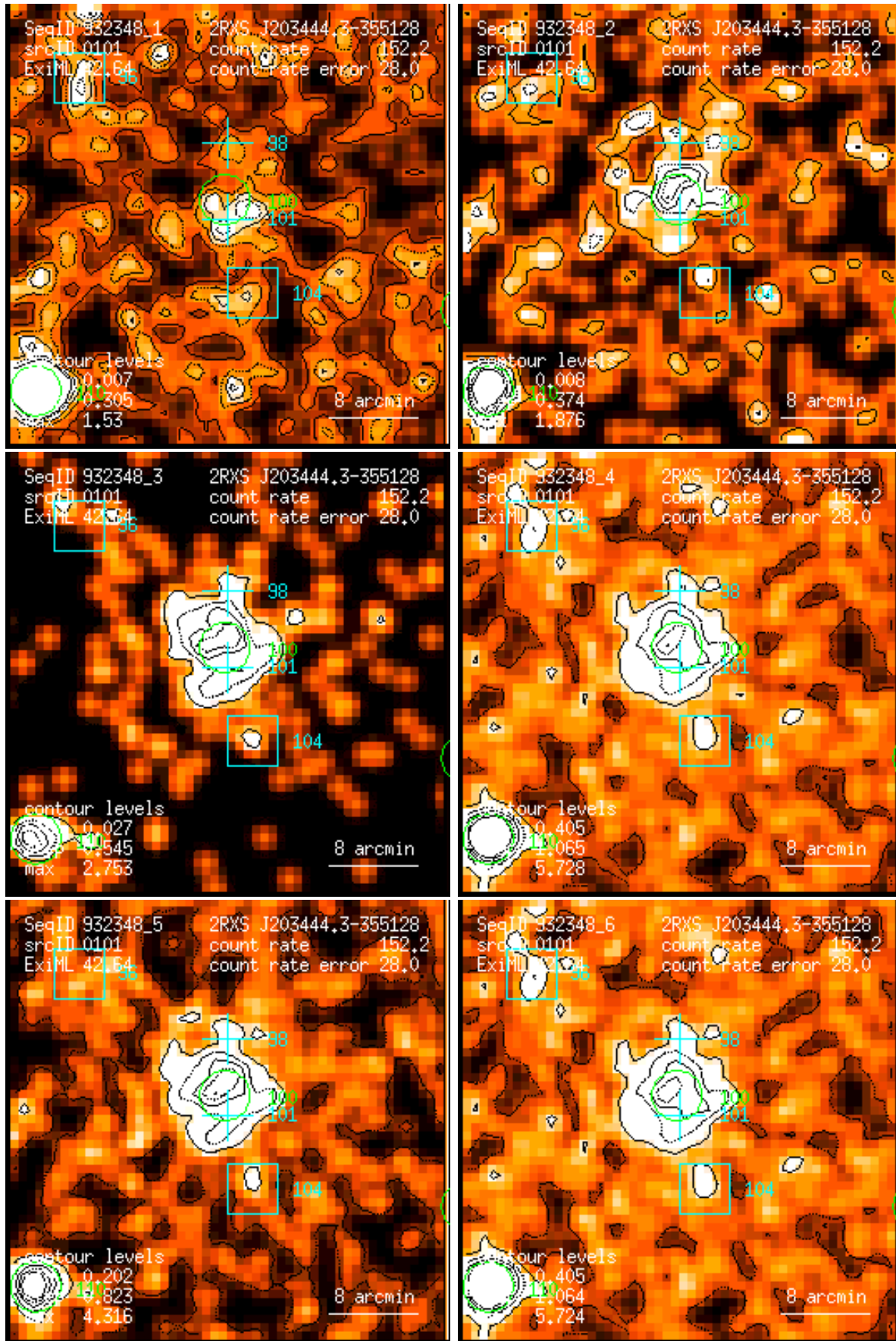
Figure 101: RASS 932348: detection 0101: band rate images, Gaussian filter: (1) PSPC channels 11 – 41, (2) 52 – 90, (3) 91 – 201, (4) 11 – 235, (5) 52 – 201, (6) 11 – 201. Broad band rates in counts/ks. Band rate contour levels in counts/ks/arcmin 2 .
