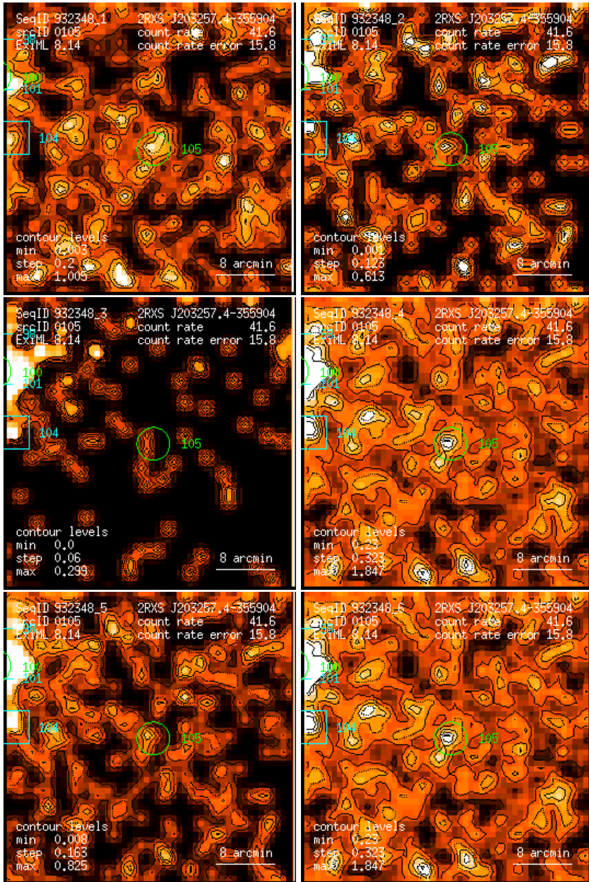
Figure 105: RASS 932348: detection 0105: band rate images, Gaussian filter: (1) PSPC channels 11 – 41, (2) 52 – 90, (3) 91 – 201, (4) 11 – 235, (5) 52 – 201, (6) 11 – 201. Broad band rates in counts/ks. Band rate contour levels in counts/ks/arcmin 2 .
