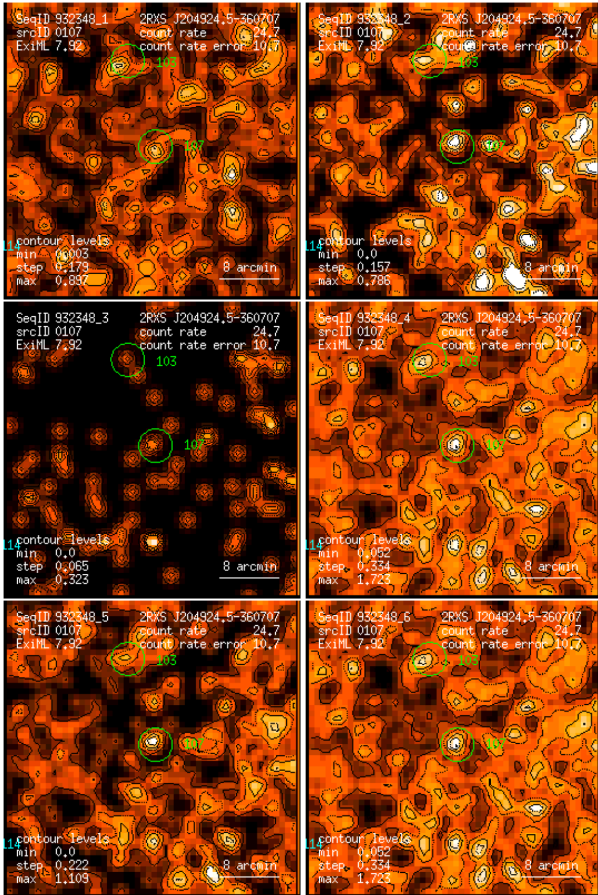
Figure 107: RASS 932348: detection 0107: band rate images, Gaussian filter: (1) PSPC channels 11 – 41, (2) 52 – 90, (3) 91 – 201, (4) 11 – 235, (5) 52 – 201, (6) 11 – 201. Broad band rates in counts/ks. Band rate contour levels in counts/ks/arcmin 2 .
