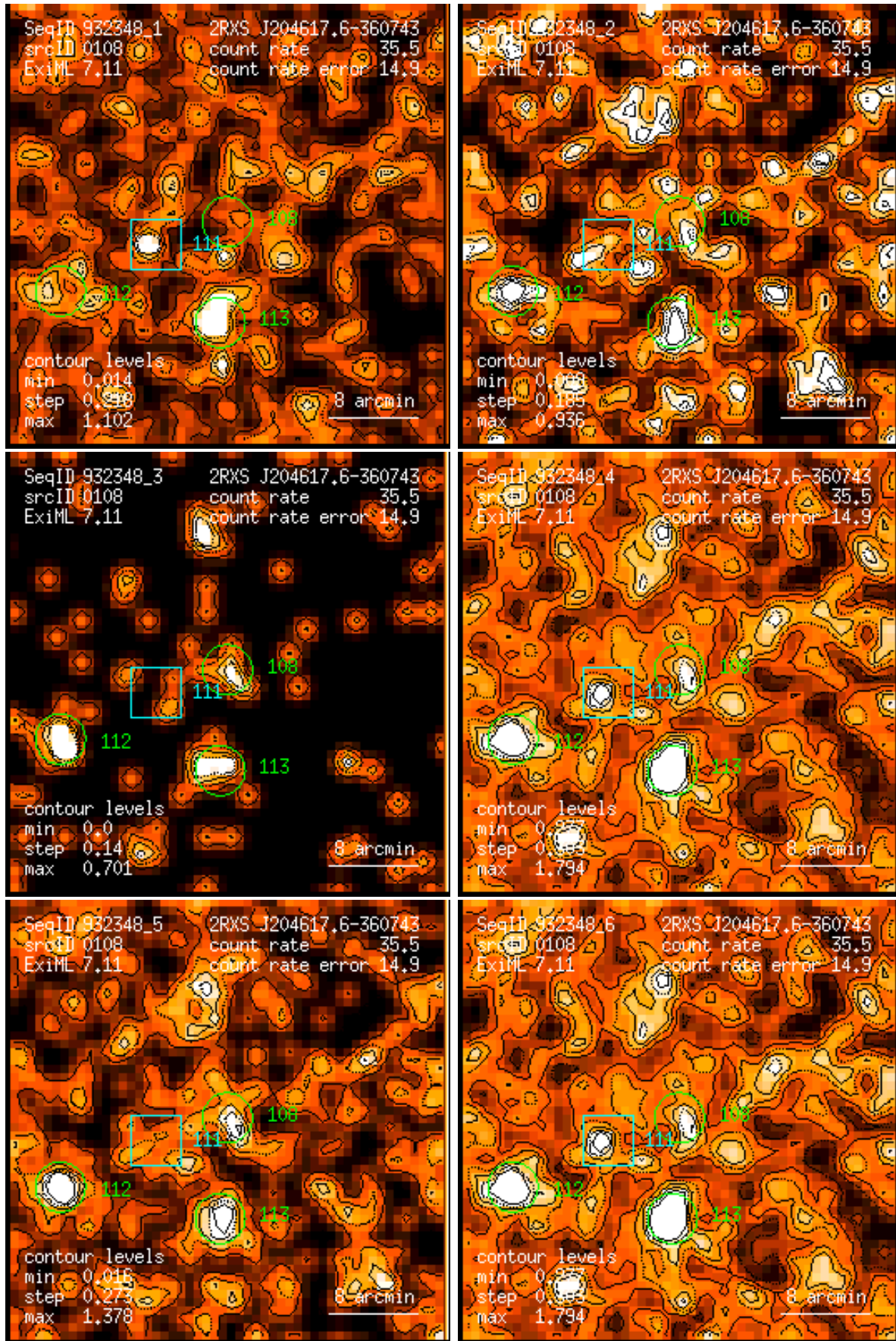
Figure 108: RASS 932348: detection 0108: band rate images, Gaussian filter: (1) PSPC channels 11 – 41, (2) 52 – 90, (3) 91 – 201, (4) 11 – 235, (5) 52 – 201, (6) 11 – 201. Broad band rates in counts/ks. Band rate contour levels in counts/ks/arcmin 2 .
