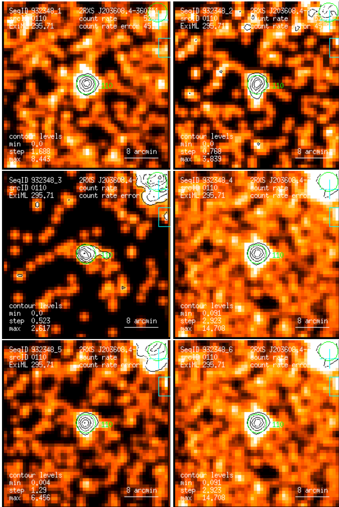
Figure 110: RASS 932348: detection 0110: band rate images, Gaussian filter: (1) PSPC channels 11 – 41, (2) 52 – 90, (3) 91 – 201, (4) 11 – 235, (5) 52 – 201, (6) 11 – 201. Broad band rates in counts/ks. Band rate contour levels in counts/ks/arcmin 2 .
