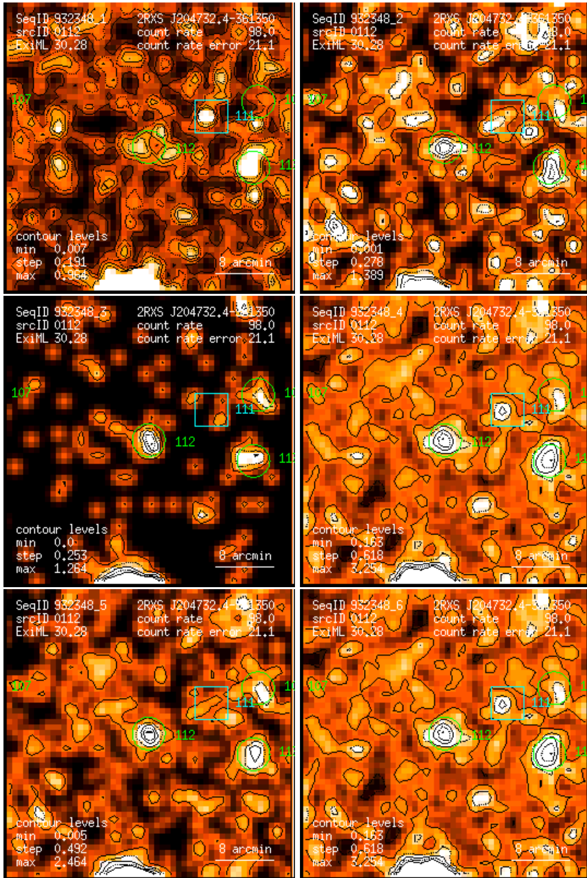
Figure 112: RASS 932348: detection 0112: band rate images, Gaussian filter: (1) PSPC channels 11 – 41, (2) 52 – 90, (3) 91 – 201, (4) 11 – 235, (5) 52 – 201, (6) 11 – 201. Broad band rates in counts/ks. Band rate contour levels in counts/ks/arcmin 2 .
