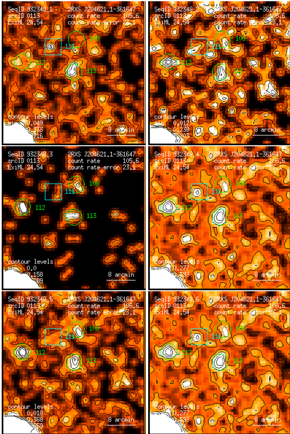
Figure 113: RASS 932348: detection 0113: band rate images, Gaussian filter: (1) PSPC channels 11 – 41, (2) 52 – 90, (3) 91 – 201, (4) 11 – 235, (5) 52 – 201, (6) 11 – 201. Broad band rates in counts/ks. Band rate contour levels in counts/ks/arcmin 2 .
