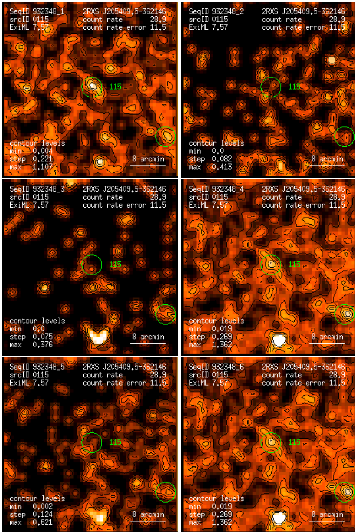
Figure 115: RASS 932348: detection 0115: band rate images, Gaussian filter: (1) PSPC channels 11 – 41, (2) 52 – 90, (3) 91 – 201, (4) 11 – 235, (5) 52 – 201, (6) 11 – 201. Broad band rates in counts/ks. Band rate contour levels in counts/ks/arcmin 2 .
