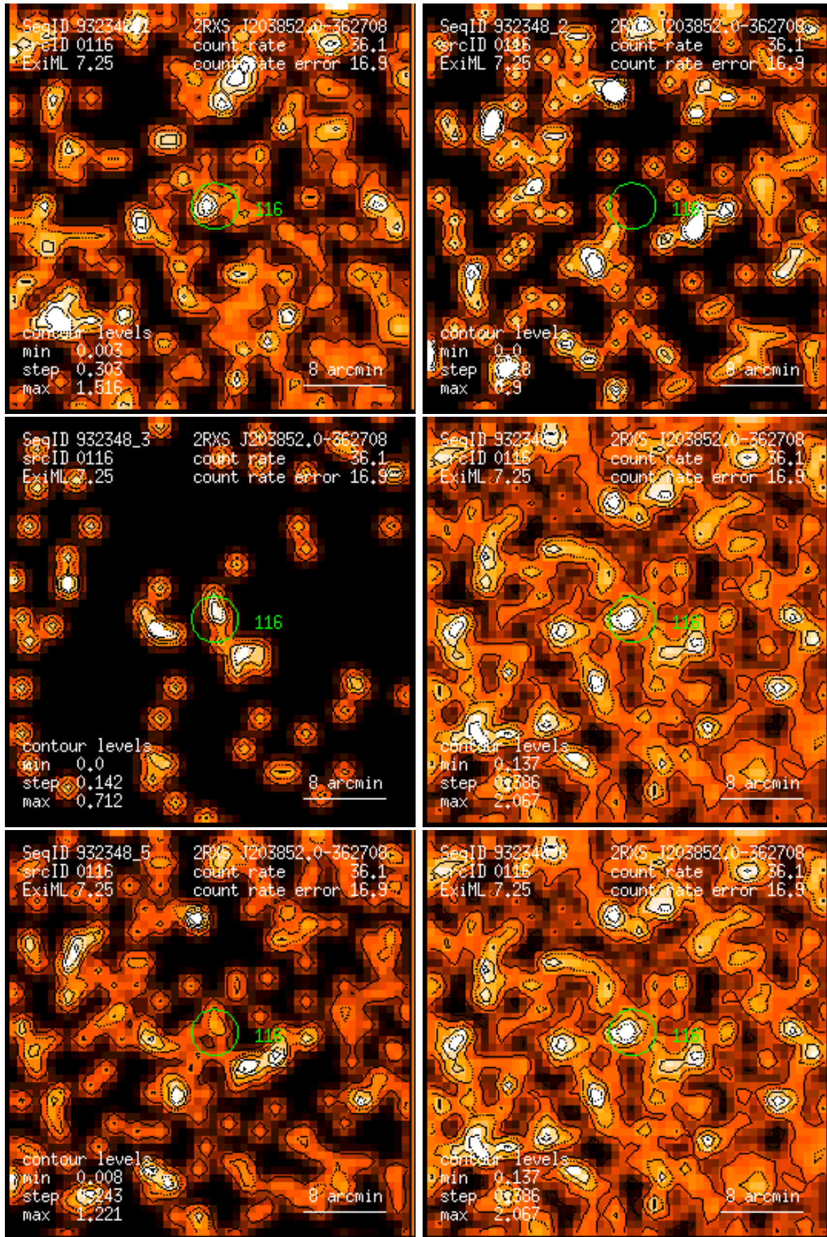
Figure 116: RASS 932348: detection 0116: band rate images, Gaussian filter: (1) PSPC channels 11 – 41, (2) 52 – 90, (3) 91 – 201, (4) 11 – 235, (5) 52 – 201, (6) 11 – 201. Broad band rates in counts/ks. Band rate contour levels in counts/ks/arcmin 2 .
