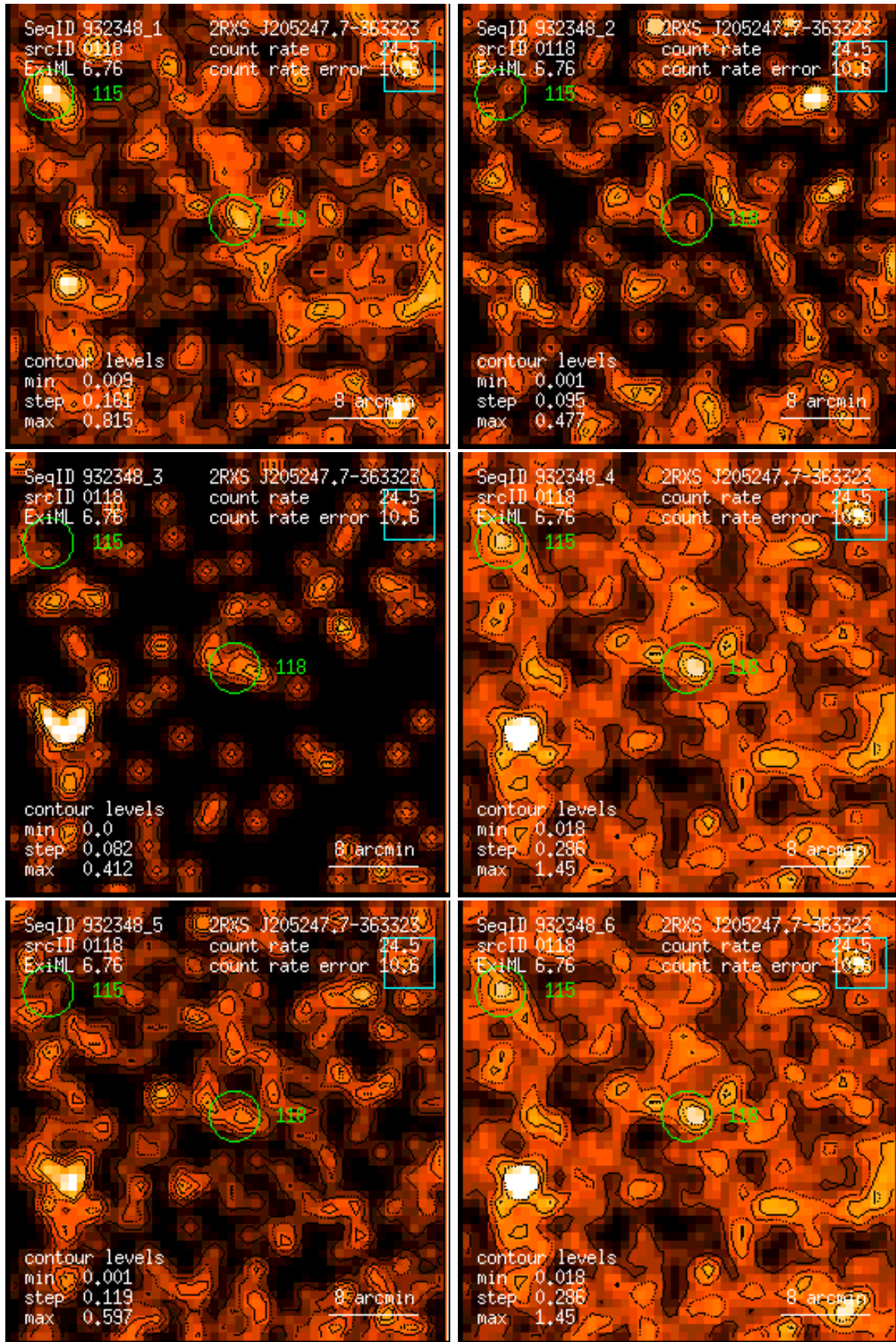
Figure 118: RASS 932348: detection 0118: band rate images, Gaussian filter: (1) PSPC channels 11 – 41, (2) 52 – 90, (3) 91 – 201, (4) 11 – 235, (5) 52 – 201, (6) 11 – 201. Broad band rates in counts/ks. Band rate contour levels in counts/ks/arcmin 2 .
