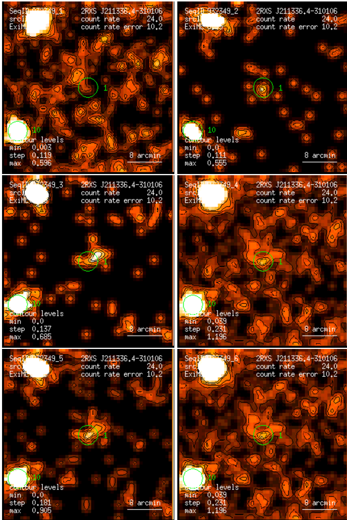
Figure 1: RASS 932349: detection 0001: band rate images, Gaussian filter: (1) PSPC channels 11 – 41, (2) 52 – 90, (3) 91 – 201, (4) 11 – 235, (5) 52 – 201, (6) 11 – 201. Broad band rates in counts/ks. Band rate contour levels in counts/ks/arcmin 2 .
