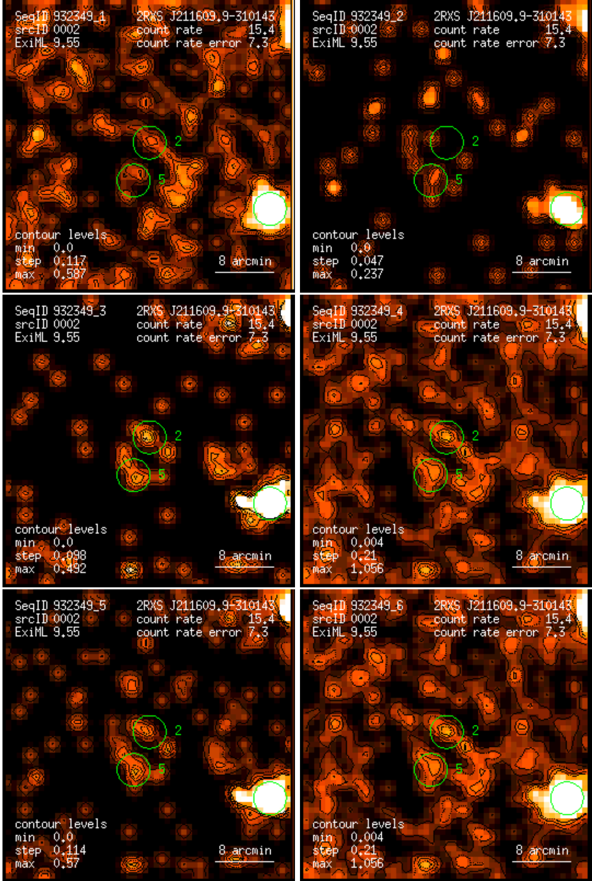
Figure 2: RASS 932349: detection 0002: band rate images, Gaussian filter: (1) PSPC channels 11 – 41, (2) 52 – 90, (3) 91 – 201, (4) 11 – 235, (5) 52 – 201, (6) 11 – 201. Broad band rates in counts/ks. Band rate contour levels in counts/ks/arcmin 2 .
