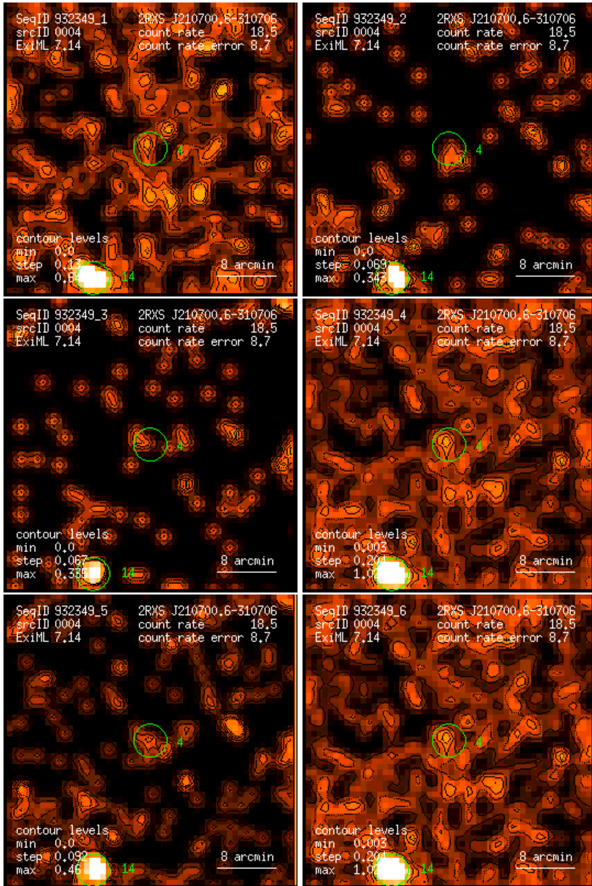
Figure 4: RASS 932349: detection 0004: band rate images, Gaussian filter: (1) PSPC channels 11 – 41, (2) 52 – 90, (3) 91 – 201, (4) 11 – 235, (5) 52 – 201, (6) 11 – 201. Broad band rates in counts/ks. Band rate contour levels in counts/ks/arcmin 2 .
