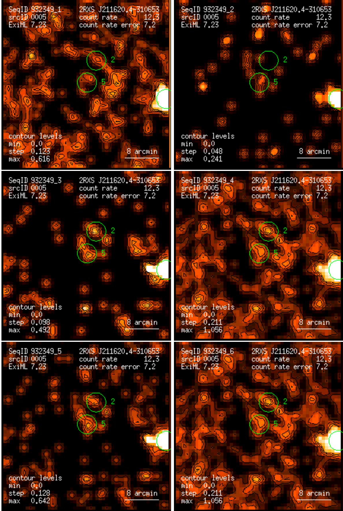
Figure 5: RASS 932349: detection 0005: band rate images, Gaussian filter: (1) PSPC channels 11 – 41, (2) 52 – 90, (3) 91 – 201, (4) 11 – 235, (5) 52 – 201, (6) 11 – 201. Broad band rates in counts/ks. Band rate contour levels in counts/ks/arcmin 2 .
