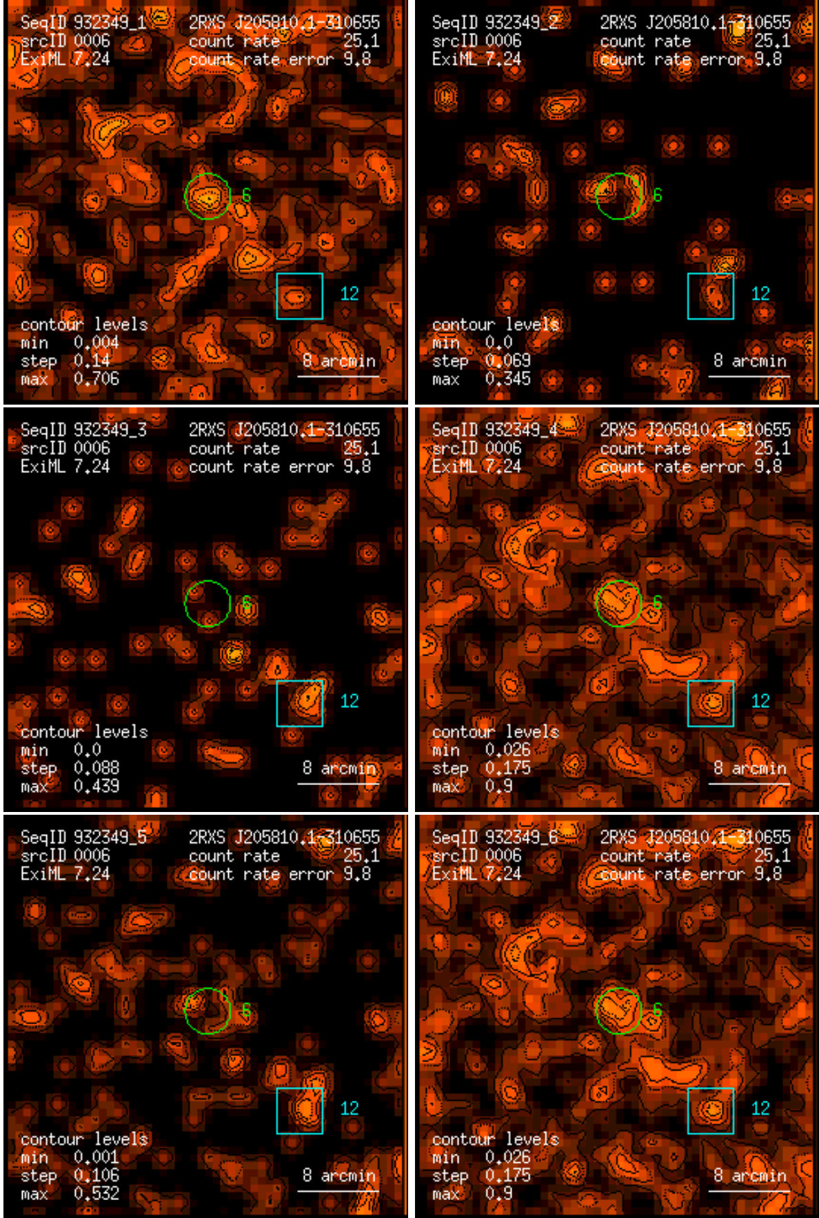
Figure 6: RASS 932349: detection 0006: band rate images, Gaussian filter: (1) PSPC channels 11 – 41, (2) 52 – 90, (3) 91 – 201, (4) 11 – 235, (5) 52 – 201, (6) 11 – 201. Broad band rates in counts/ks. Band rate contour levels in counts/ks/arcmin 2 .
