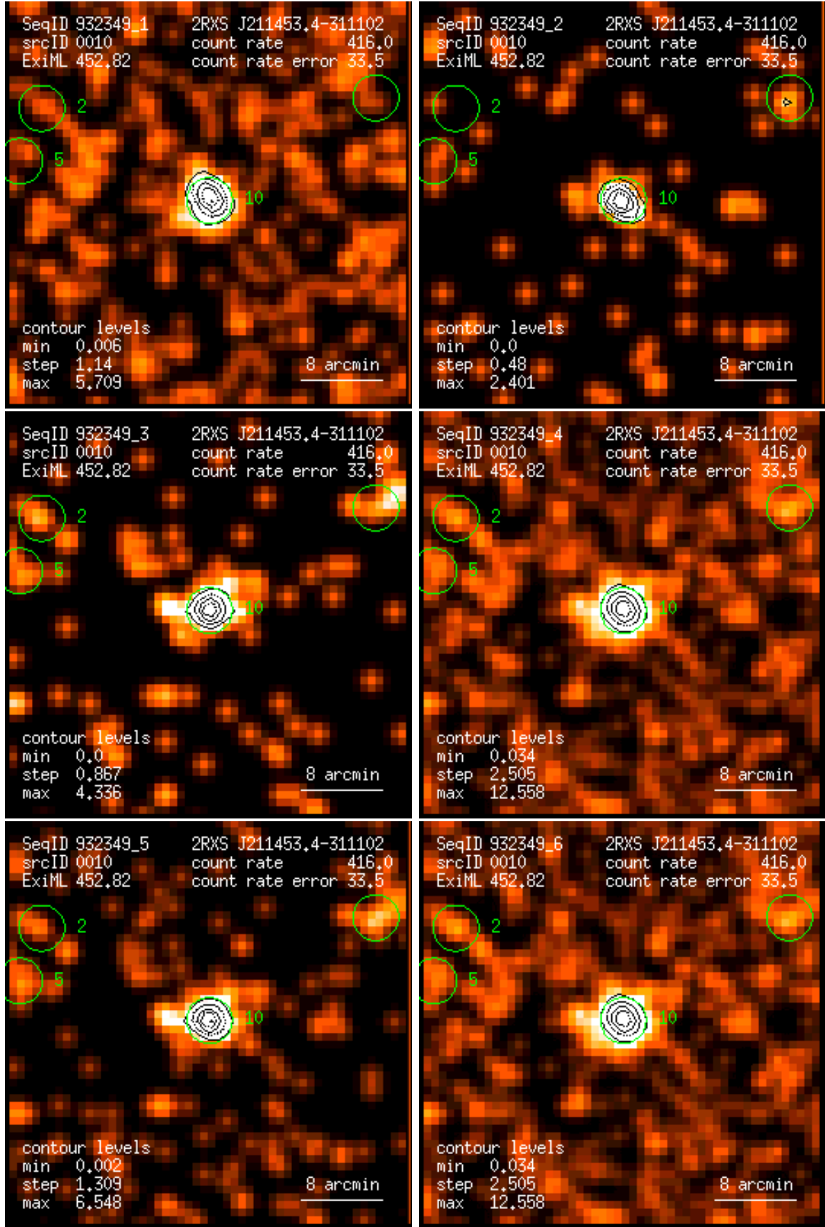
Figure 10: RASS 932349: detection 0010: band rate images, Gaussian filter: (1) PSPC channels 11 – 41, (2) 52 – 90, (3) 91 – 201, (4) 11 – 235, (5) 52 – 201, (6) 11 – 201. Broad band rates in counts/ks. Band rate contour levels in counts/ks/arcmin 2 .
