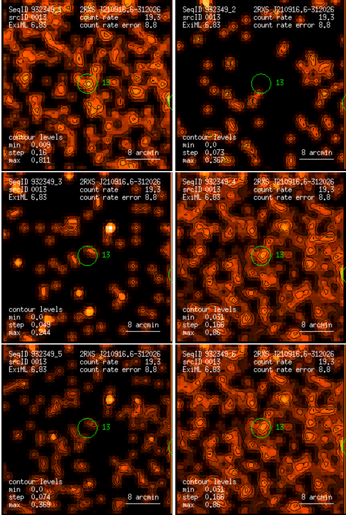
Figure 13: RASS 932349: detection 0013: band rate images, Gaussian filter: (1) PSPC channels 11 – 41, (2) 52 – 90, (3) 91 – 201, (4) 11 – 235, (5) 52 – 201, (6) 11 – 201. Broad band rates in counts/ks. Band rate contour levels in counts/ks/arcmin 2 .
