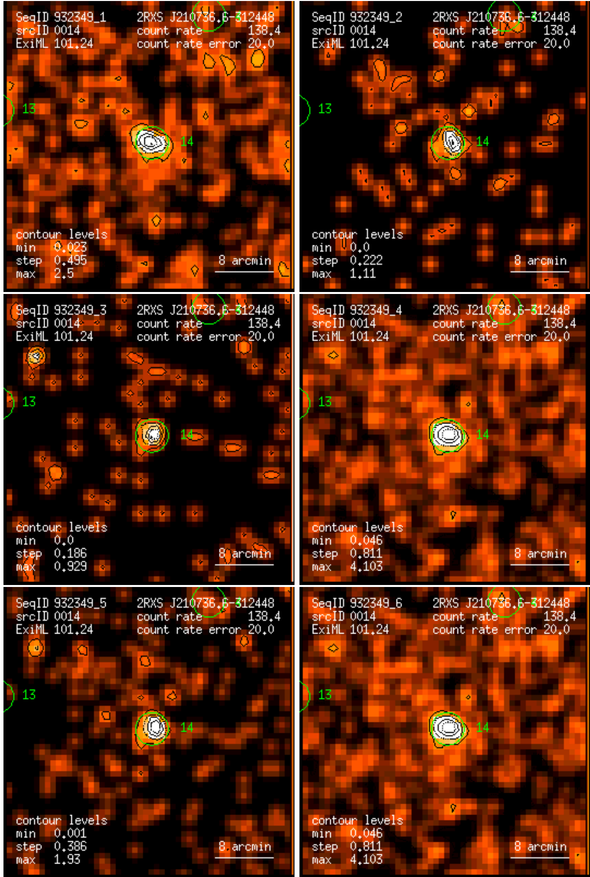
Figure 14: RASS 932349: detection 0014: band rate images, Gaussian filter: (1) PSPC channels 11 – 41, (2) 52 – 90, (3) 91 – 201, (4) 11 – 235, (5) 52 – 201, (6) 11 – 201. Broad band rates in counts/ks. Band rate contour levels in counts/ks/arcmin 2 .
