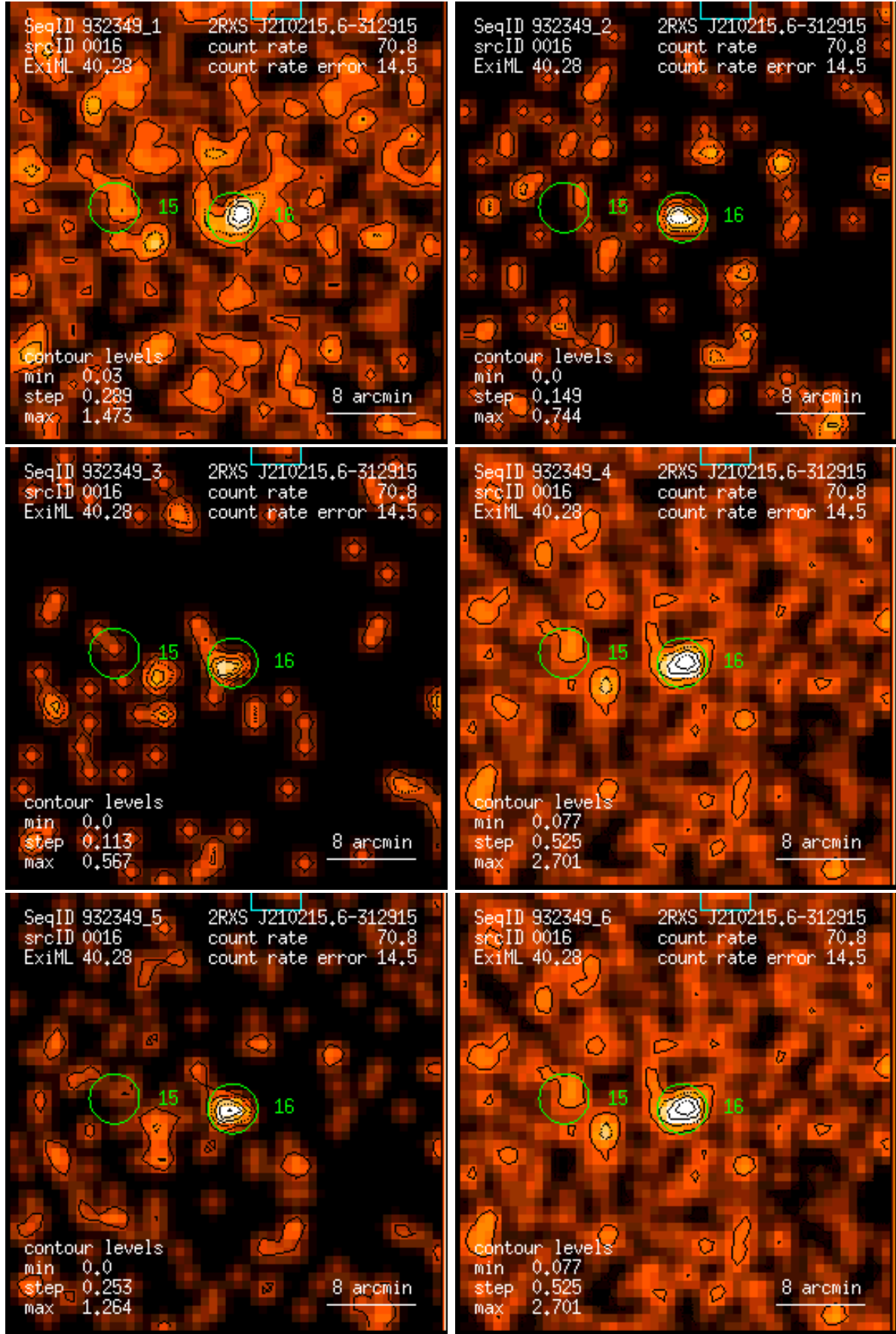
Figure 16: RASS 932349: detection 0016: band rate images, Gaussian filter: (1) PSPC channels 11 – 41, (2) 52 – 90, (3) 91 – 201, (4) 11 – 235, (5) 52 – 201, (6) 11 – 201. Broad band rates in counts/ks. Band rate contour levels in counts/ks/arcmin 2 .
