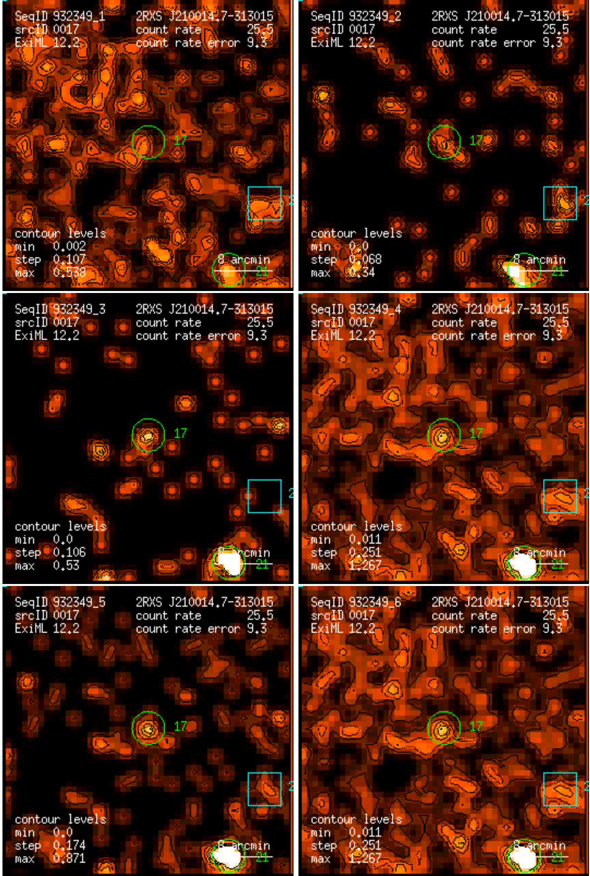
Figure 17: RASS 932349: detection 0017: band rate images, Gaussian filter: (1) PSPC channels 11 – 41, (2) 52 – 90, (3) 91 – 201, (4) 11 – 235, (5) 52 – 201, (6) 11 – 201. Broad band rates in counts/ks. Band rate contour levels in counts/ks/arcmin 2 .
