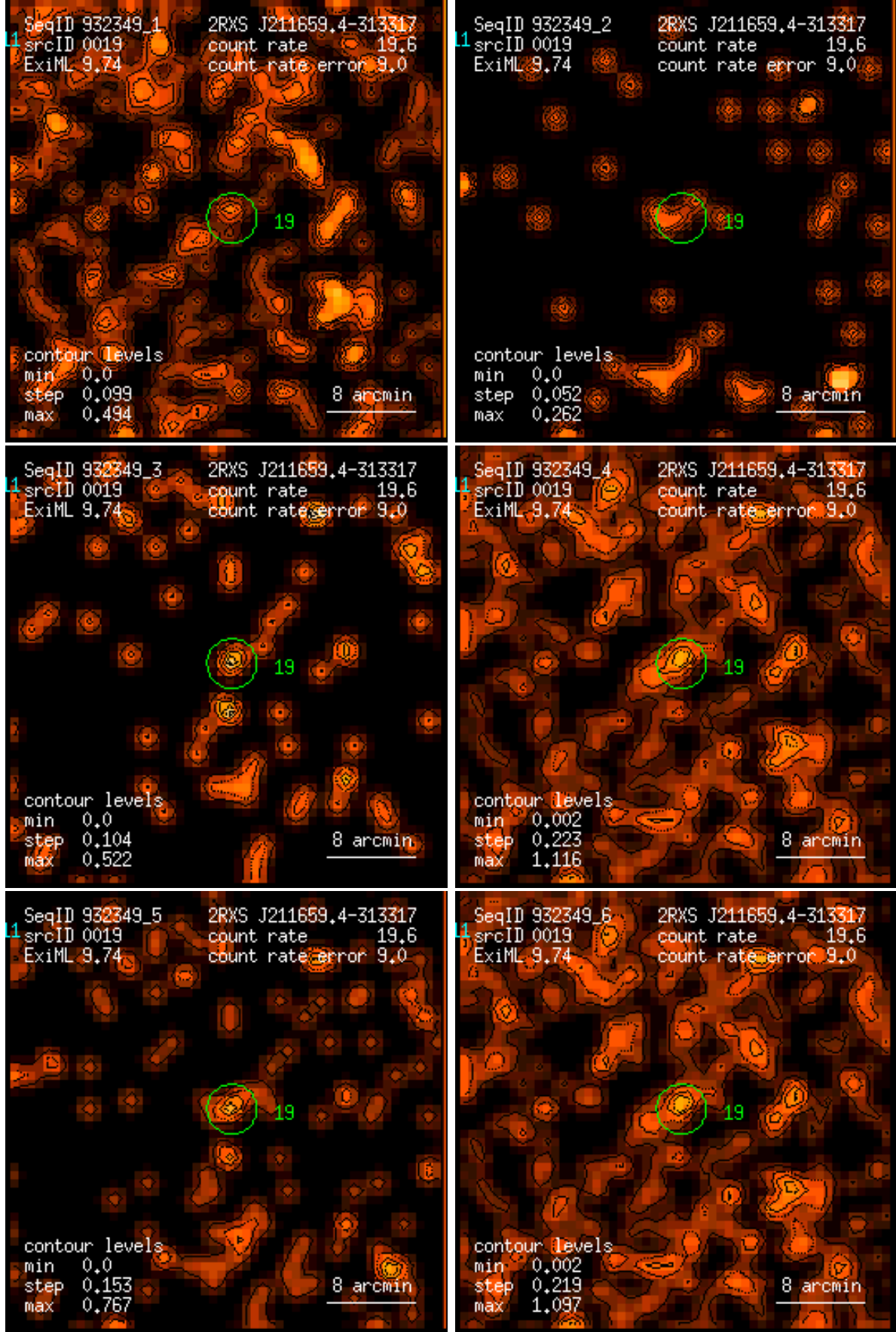
Figure 19: RASS 932349: detection 0019: band rate images, Gaussian filter: (1) PSPC channels 11 – 41, (2) 52 – 90, (3) 91 – 201, (4) 11 – 235, (5) 52 – 201, (6) 11 – 201. Broad band rates in counts/ks. Band rate contour levels in counts/ks/arcmin 2 .
