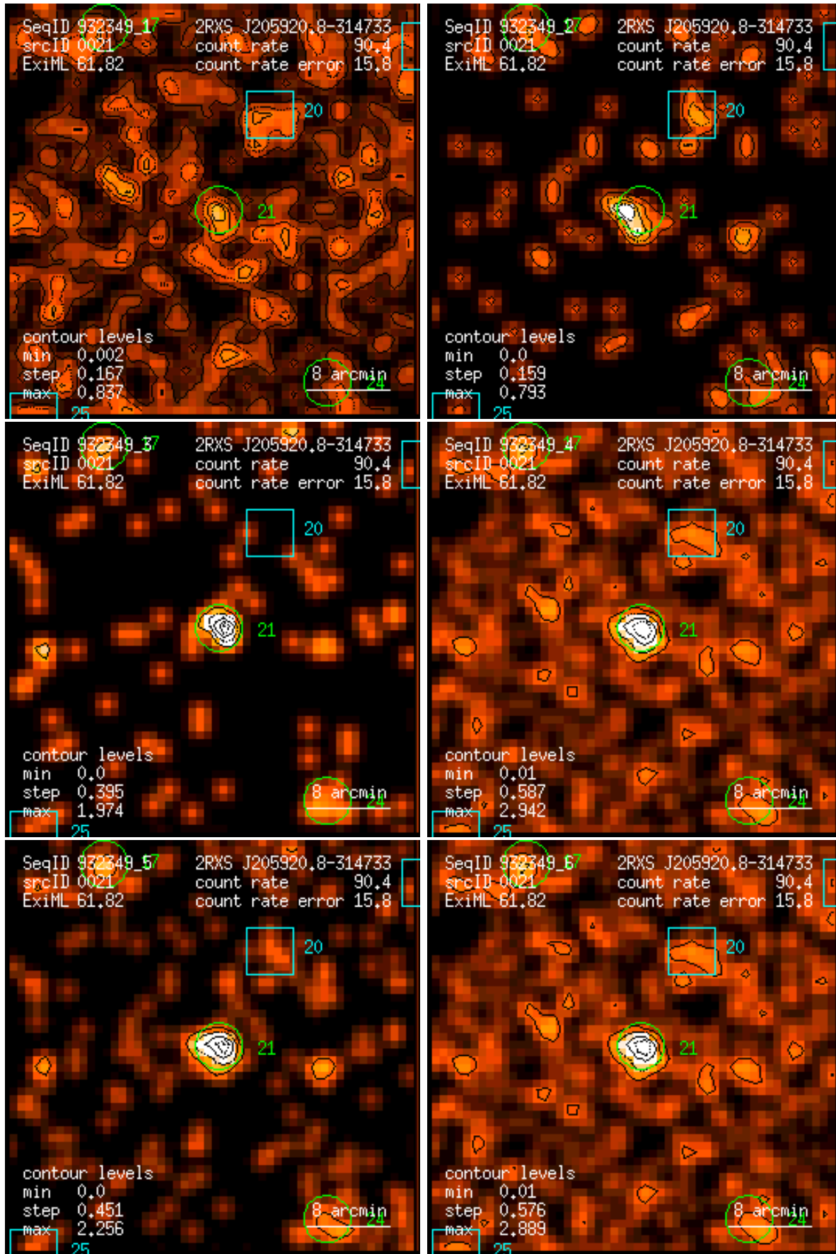
Figure 21: RASS 932349: detection 0021: band rate images, Gaussian filter: (1) PSPC channels 11 – 41, (2) 52 – 90, (3) 91 – 201, (4) 11 – 235, (5) 52 – 201, (6) 11 – 201. Broad band rates in counts/ks. Band rate contour levels in counts/ks/arcmin 2 .
