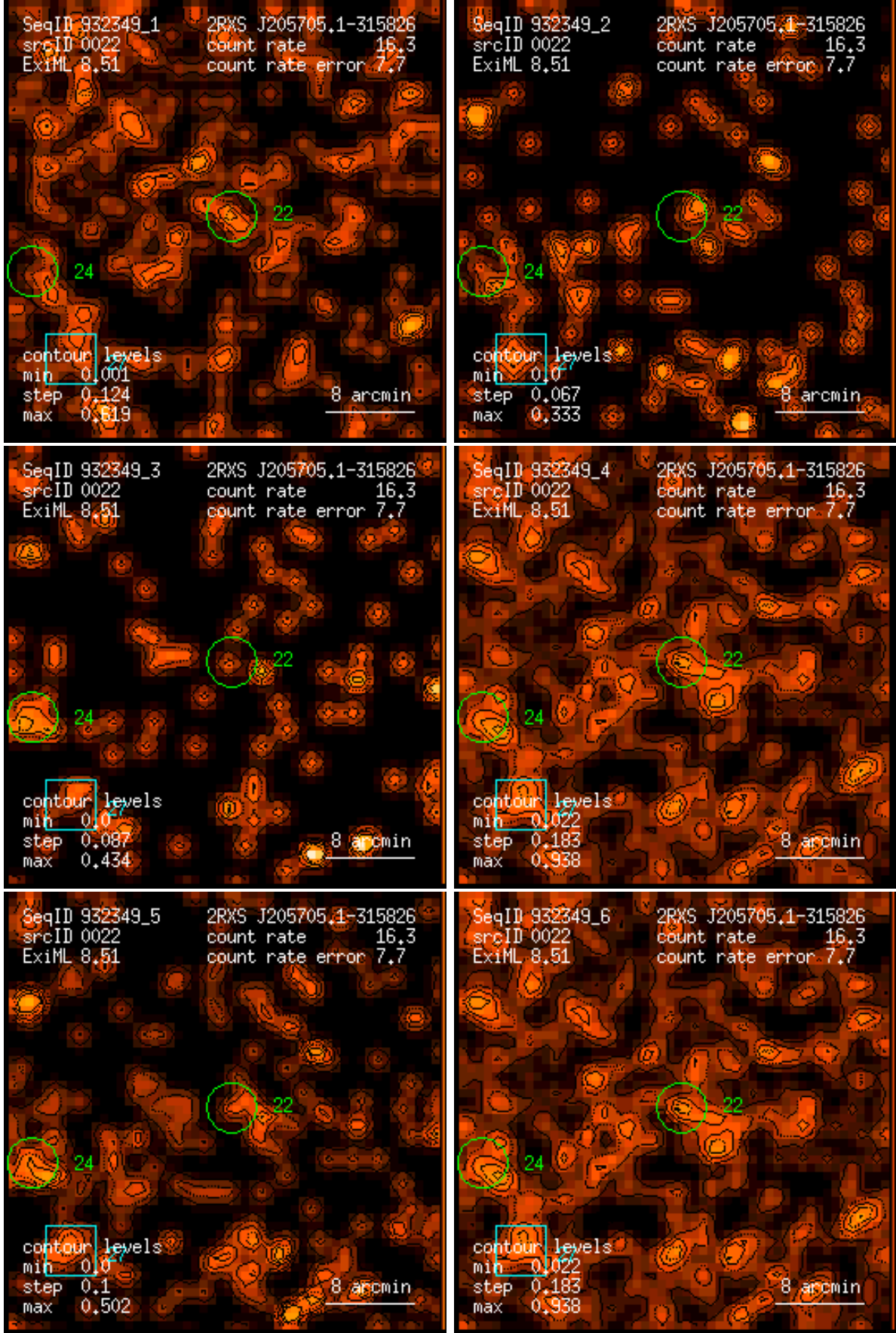
Figure 22: RASS 932349: detection 0022: band rate images, Gaussian filter: (1) PSPC channels 11 – 41, (2) 52 – 90, (3) 91 – 201, (4) 11 – 235, (5) 52 – 201, (6) 11 – 201. Broad band rates in counts/ks. Band rate contour levels in counts/ks/arcmin 2 .
