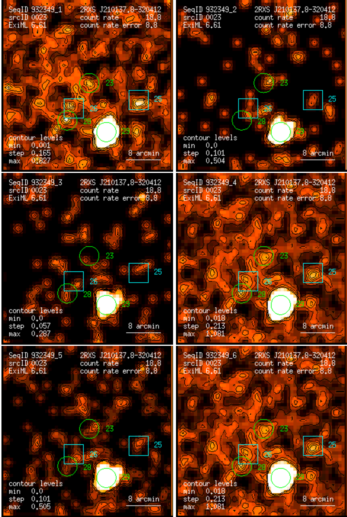
Figure 23: RASS 932349: detection 0023: band rate images, Gaussian filter: (1) PSPC channels 11 – 41, (2) 52 – 90, (3) 91 – 201, (4) 11 – 235, (5) 52 – 201, (6) 11 – 201. Broad band rates in counts/ks. Band rate contour levels in counts/ks/arcmin 2 .
