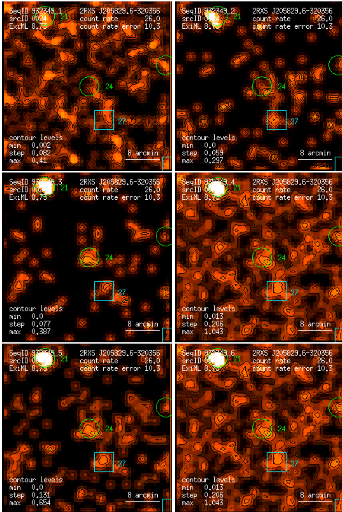
Figure 24: RASS 932349: detection 0024: band rate images, Gaussian filter: (1) PSPC channels 11 – 41, (2) 52 – 90, (3) 91 – 201, (4) 11 – 235, (5) 52 – 201, (6) 11 – 201. Broad band rates in counts/ks. Band rate contour levels in counts/ks/arcmin 2 .
