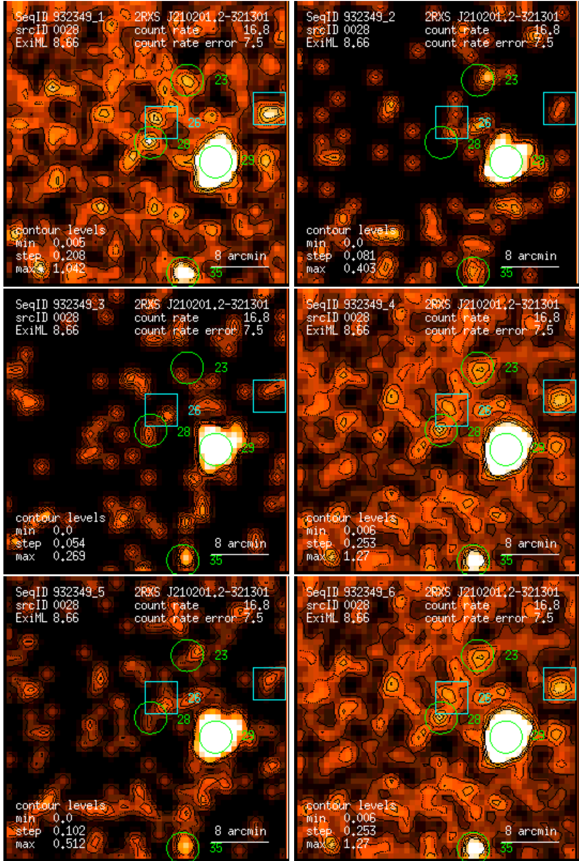
Figure 28: RASS 932349: detection 0028: band rate images, Gaussian filter: (1) PSPC channels 11 – 41, (2) 52 – 90, (3) 91 – 201, (4) 11 – 235, (5) 52 – 201, (6) 11 – 201. Broad band rates in counts/ks. Band rate contour levels in counts/ks/arcmin 2 .
