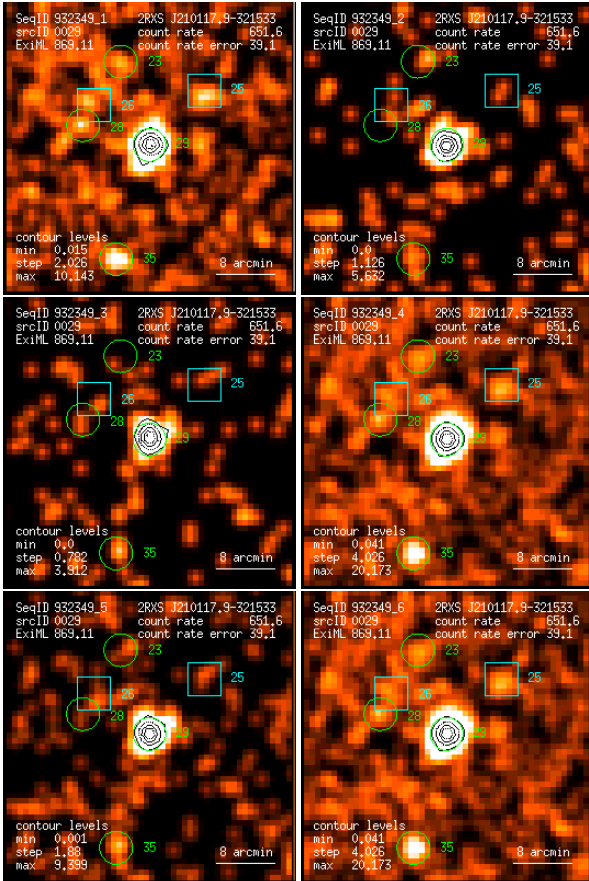
Figure 29: RASS 932349: detection 0029: band rate images, Gaussian filter: (1) PSPC channels 11 – 41, (2) 52 – 90, (3) 91 – 201, (4) 11 – 235, (5) 52 – 201, (6) 11 – 201. Broad band rates in counts/ks. Band rate contour levels in counts/ks/arcmin 2 .
