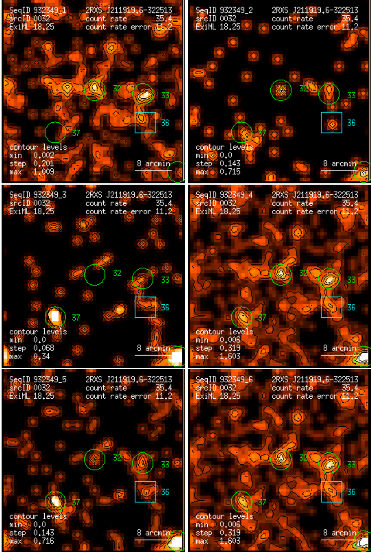
Figure 32: RASS 932349: detection 0032: band rate images, Gaussian filter: (1) PSPC channels 11 – 41, (2) 52 – 90, (3) 91 – 201, (4) 11 – 235, (5) 52 – 201, (6) 11 – 201. Broad band rates in counts/ks. Band rate contour levels in counts/ks/arcmin 2 .
