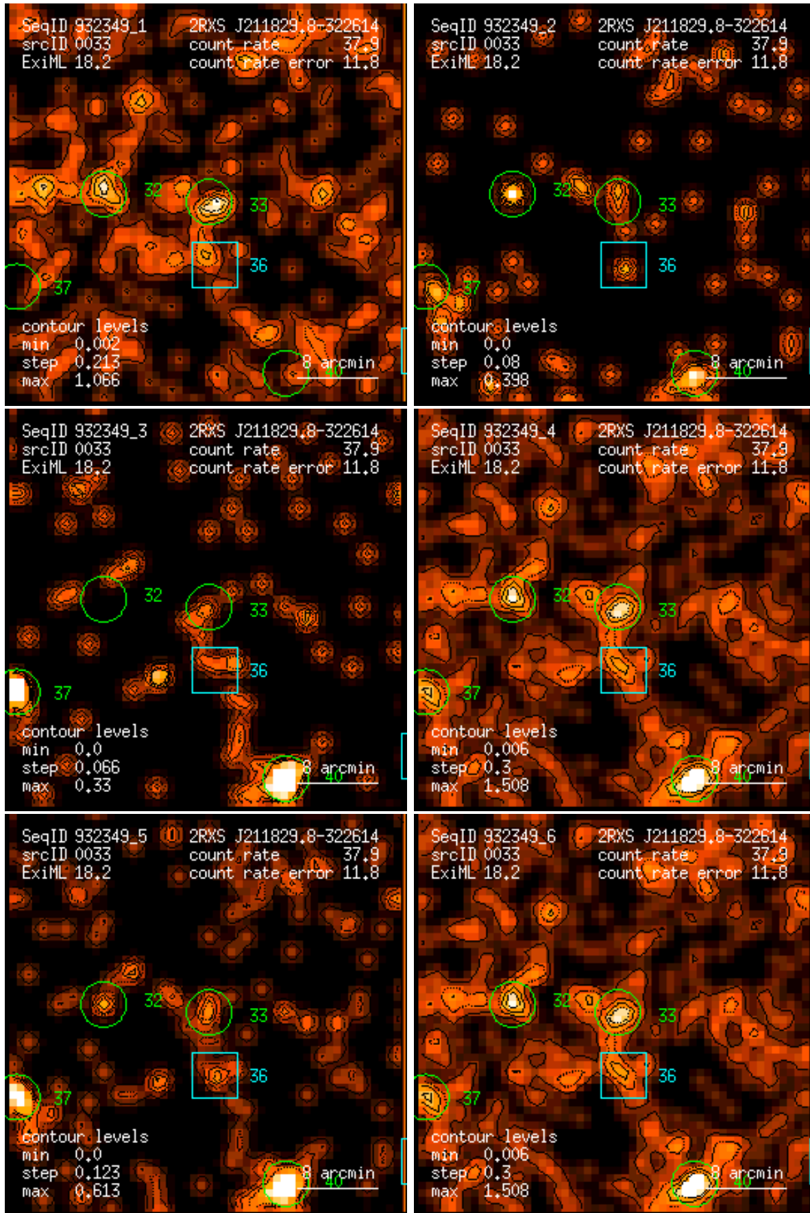
Figure 33: RASS 932349: detection 0033: band rate images, Gaussian filter: (1) PSPC channels 11 – 41, (2) 52 – 90, (3) 91 – 201, (4) 11 – 235, (5) 52 – 201, (6) 11 – 201. Broad band rates in counts/ks. Band rate contour levels in counts/ks/arcmin 2 .
