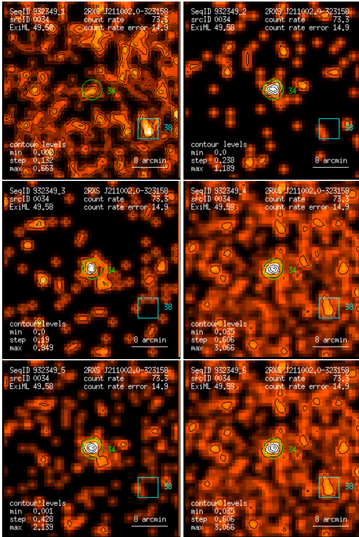
Figure 34: RASS 932349: detection 0034: band rate images, Gaussian filter: (1) PSPC channels 11 – 41, (2) 52 – 90, (3) 91 – 201, (4) 11 – 235, (5) 52 – 201, (6) 11 – 201. Broad band rates in counts/ks. Band rate contour levels in counts/ks/arcmin 2 .
