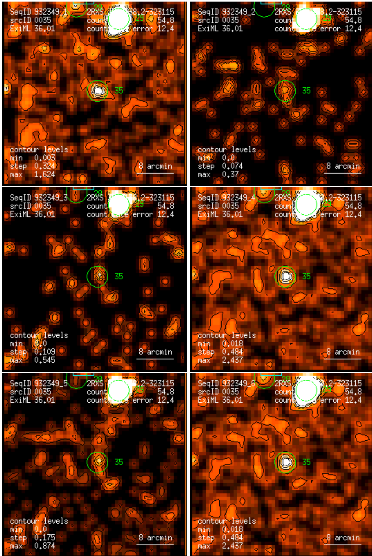
Figure 35: RASS 932349: detection 0035: band rate images, Gaussian filter: (1) PSPC channels 11 – 41, (2) 52 – 90, (3) 91 – 201, (4) 11 – 235, (5) 52 – 201, (6) 11 – 201. Broad band rates in counts/ks. Band rate contour levels in counts/ks/arcmin 2 .
