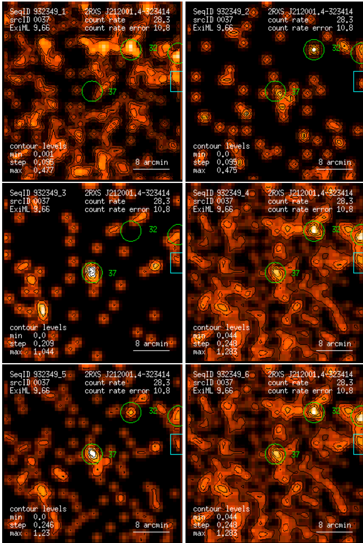
Figure 37: RASS 932349: detection 0037: band rate images, Gaussian filter: (1) PSPC channels 11 – 41, (2) 52 – 90, (3) 91 – 201, (4) 11 – 235, (5) 52 – 201, (6) 11 – 201. Broad band rates in counts/ks. Band rate contour levels in counts/ks/arcmin 2 .
