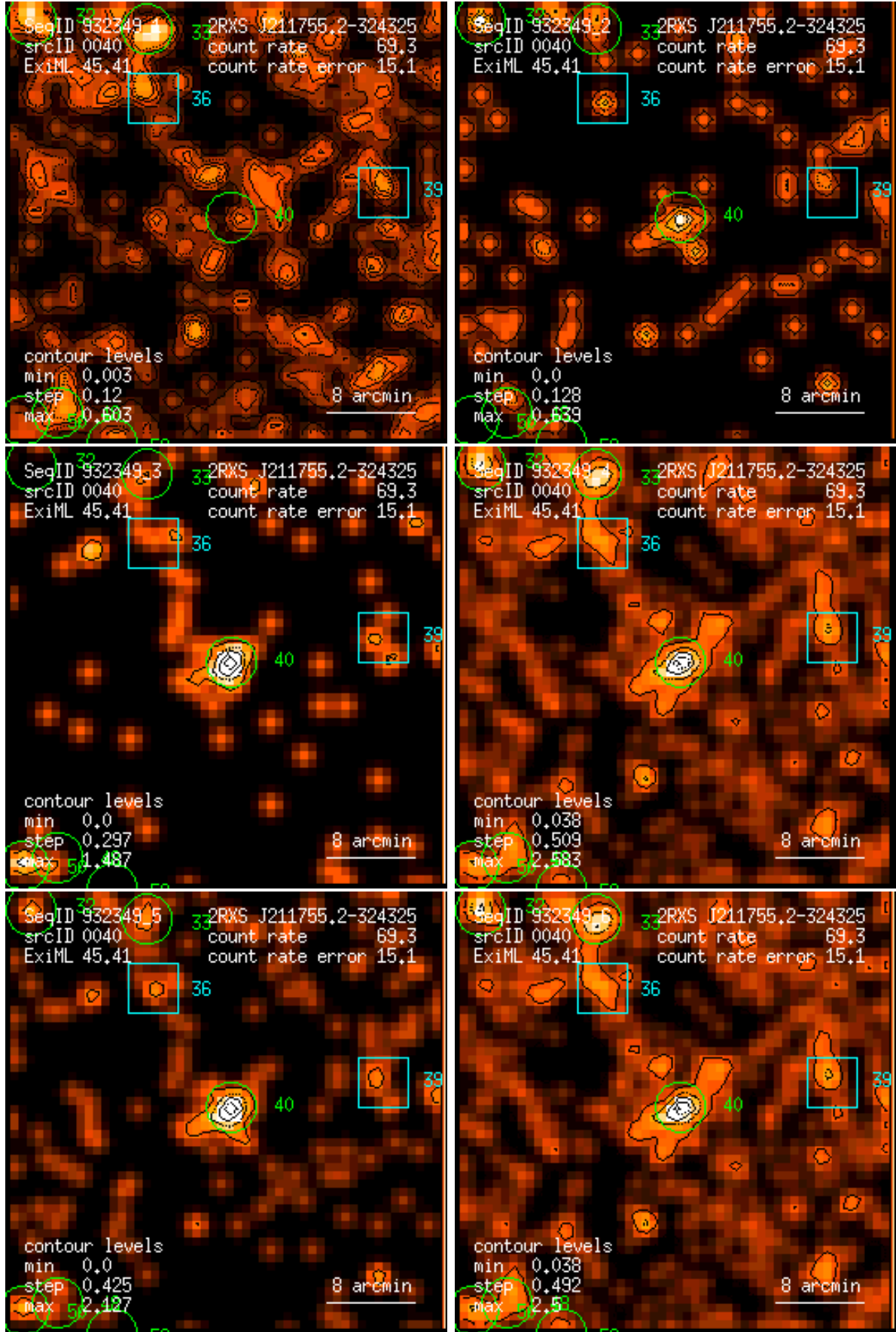
Figure 40: RASS 932349: detection 0040: band rate images, Gaussian filter: (1) PSPC channels 11 – 41, (2) 52 – 90, (3) 91 – 201, (4) 11 – 235, (5) 52 – 201, (6) 11 – 201. Broad band rates in counts/ks. Band rate contour levels in counts/ks/arcmin 2 .
